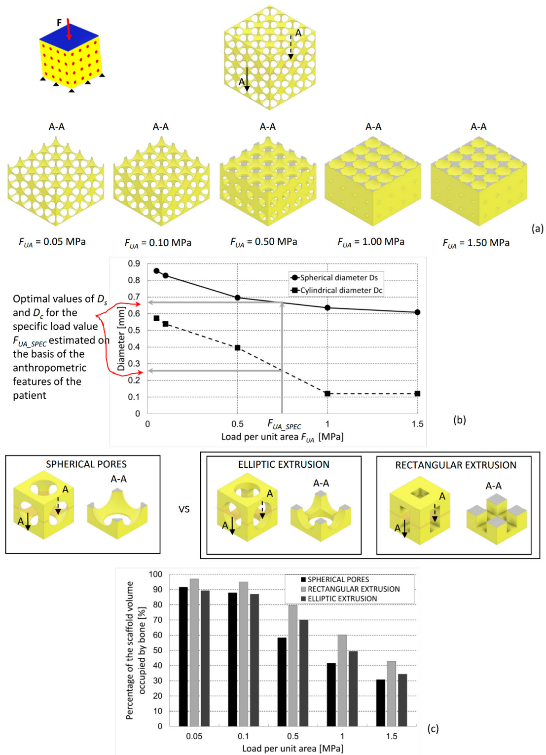
Figure 7. (a) Optimized scaffold geometries (section views A-A), (b) optimal values of D_s and D_c , and (c) percentage of the scaffold volume occupied by mature bone, predicted by the optimization algorithm for different values of the compression load. The percentages of bone are compared with those predicted for scaffolds with hexahedron unit cells including elliptic and rectangular extrusions [20].
