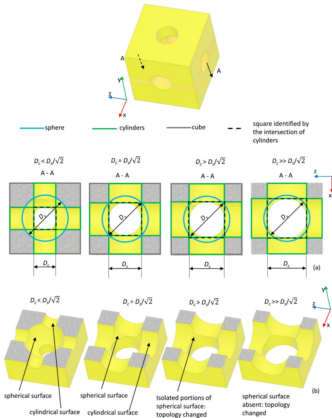
Figure 3. (a) Section views—in the plane x - z —of the scaffold unit cell (topology (S)) with indicated edges of the primitives (cube, cylinders, and sphere) utilized. When the square obtained by the intersection of the cylinders touches with its vertices, the spherical edge (in blue), the limit condition D_c = D_s/\sqrt{2} is reached. For D_c > D_s/\sqrt{2} , the topology of the unit cell changes. (b) Section views—in the three-dimensional space—of the unit cell obtained for different values of D_s and D_c .
