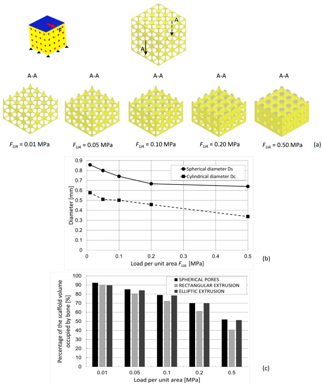
Figure 8. (a) Optimized scaffold geometries (section views A-A), (b) optimal values of D_s and D_c , and (c) percentage of the scaffold volume occupied by mature bone, predicted by the optimization algorithm for different values of the shear load. The percentages of bone are compared with those predicted for scaffolds with hexahedron unit cells including elliptic and rectangular extrusions [20].
