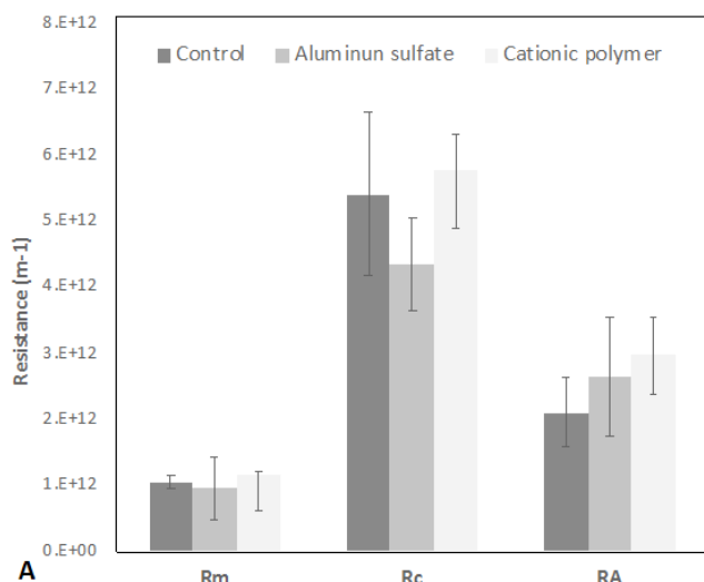
Figure 7. A - Membrane ( R_m ), cake layer ( R_c ) and adsorbed ( R_a ) resistance; B - relative contribution to the fouling resistance due to cake layer and adsorption.
