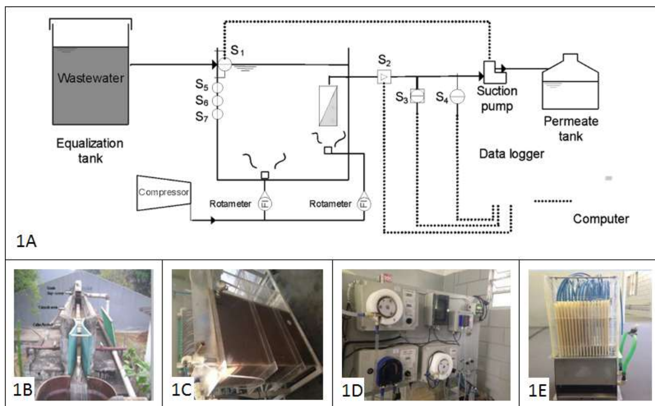
Figure 1. General view of the experimental SMBR pilot plant: 1A - Flowchart of the pilot plant; S 1 - level sensor; S 2 - permeate flow sensor; S 3 - pressure sensor; S 4 - temperature sensor; S 5 - DO probe; S 6 - pH sensor and; S 7 - ORP sensor, 1B - preliminary treatment; 1C - Membrane Bioreactor; 1D - Control Panel; 1E - Membrane Cassette.
