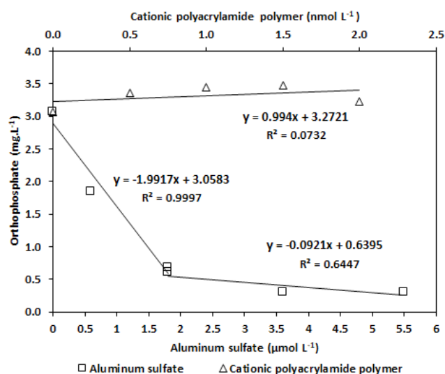
Figure 8. Orthophosphate removal relative to the coagulant and flocculant dosage.
