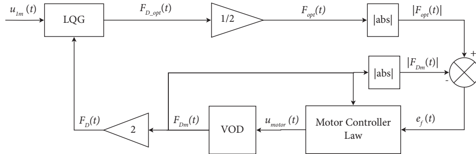
FIGURE 2: Scheme of the LQG control.
