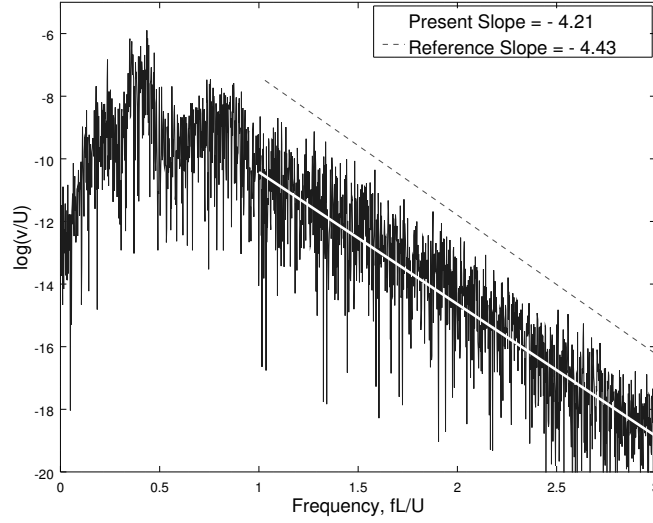
Figure 4.18: Flow past an open cavity: normalized spectrum of the scaled x_2 -component of velocity at (1.57D, 0) .
