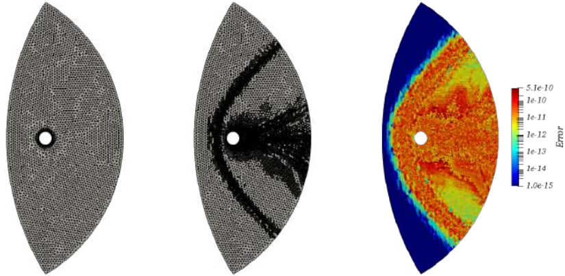
Figure 7.16: Supersonic flow past a cylinder results. Subscales-based error estimator measured with the entropy measure: initial unstructured mesh composed by 8141 P_1 elements on the left, refined mesh composed of 61020 P_1 elements on the center, and estimated error over the refined mesh on the right.
