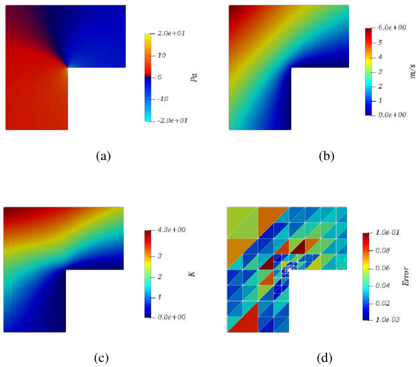
Figure 7.3: Singular exact solution results: (a) pressure contour, (b) velocity magnitude contour, (c) temperature contour, and (d) refined mesh with the subscales-based error distribution.
