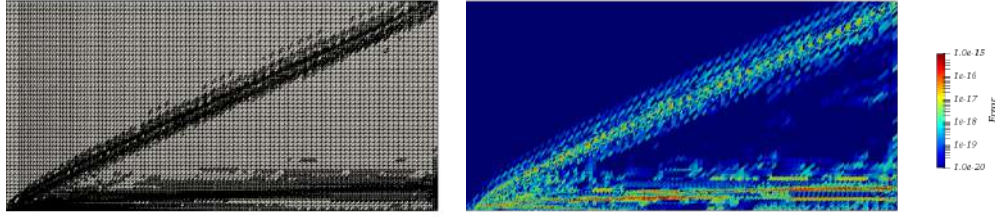
Figure 7.13: Flow over a flat plate results. Subscales-based error estimator measured with the entropy measure: refined mesh composed of 202806 elements on the left, and estimated error over the refined mesh on the right.
