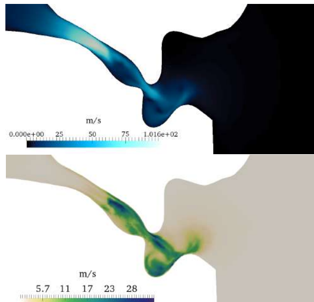
Figure 8.3: Fricative model results: time-averaged velocity magnitude (at the top), and root mean square velocity magnitude at a cutting middle plane of the constriction.
