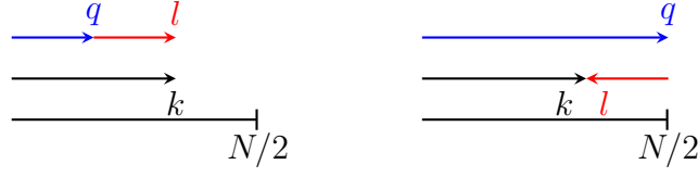
Figure 2.1: Triadic interactions among the resolved scales
