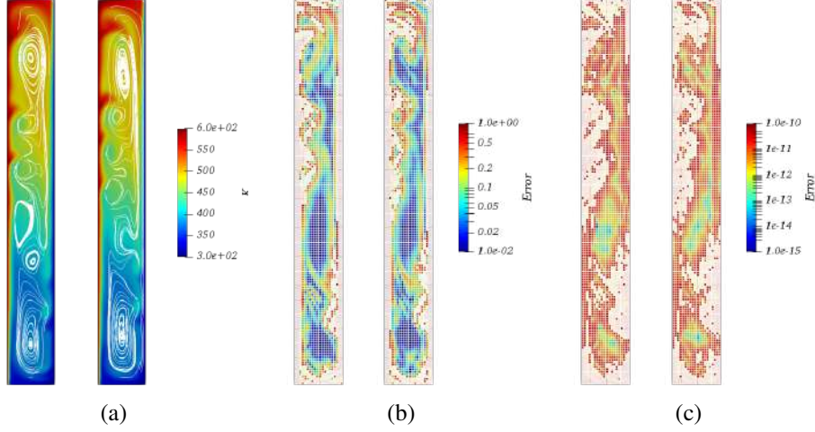
Figure 7.10: Differentially heated cavity results: (a) temperature contours with velocity streamlines, (b) scaled L^2 -norm of the variational subscales: refinement tolerance is fixed 0.1 < \eta_K^2 < 1 , which led to meshes of 6795, and 6852 elements, and (c) entropy measure of the variational subscales: refinement tolerance is fixed to 10^{-14} < \eta_K^2 < 10^{-10} , which led to meshes of 6853, and 7035 elements. Solution is obtained using the primitive formulation and it is presented for the same instants of time.
