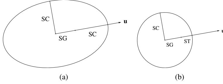
Figure 3.1: Shock capturing methods: (a) Isotropic diffusion ellipse, (b) Anisotropic diffusion ellipse.
