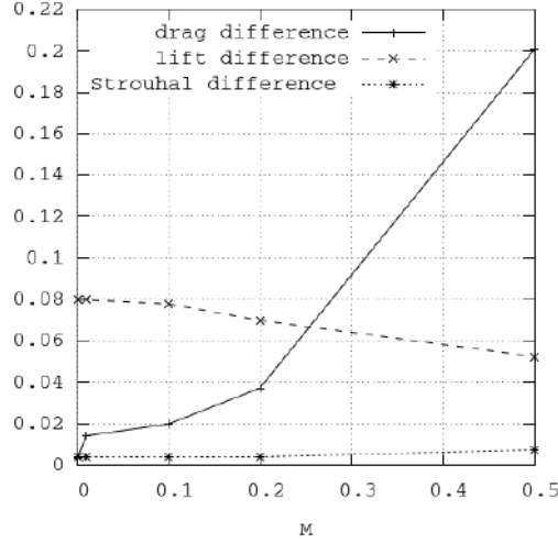
Figure 4.14: Flow past a cylinder results compared to the incompressible solution.
