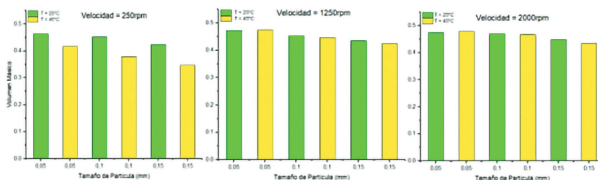
Figure 6. Mass volume in relation to fluid temperature
