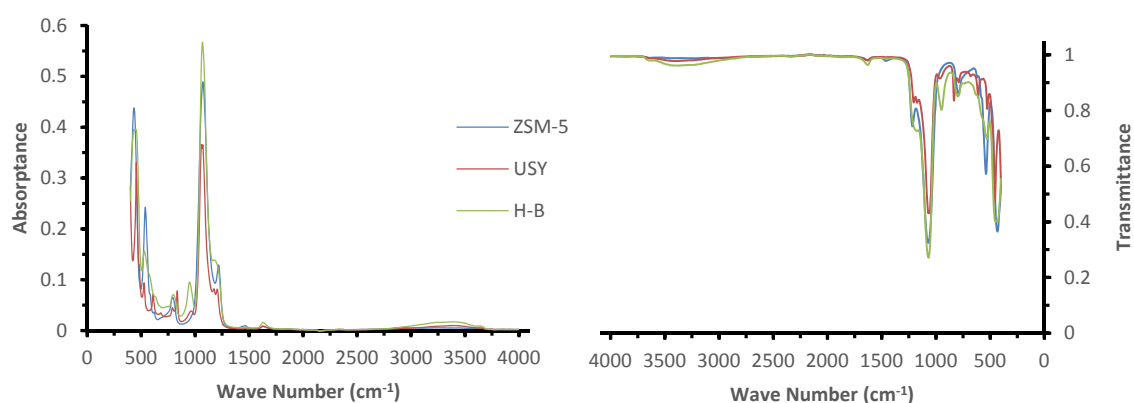
Figure 5: IR spectrum of each 1 % Pt/Zeolite catalyst.
