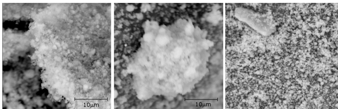
Figure 4: SEM for 1% Pt/H- \beta (left), 1% Pt/USY (center) and 1% Pt/ZSM-5 (right).
