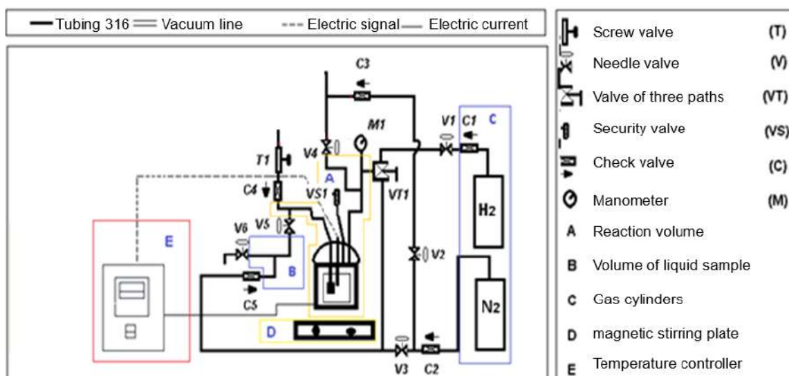
Figure 2: Reaction assembly for oil hydrotreating.
