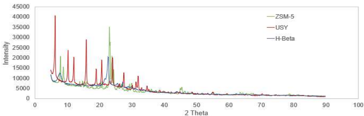
Figure 3: Diffractogram of the three catalysts.
