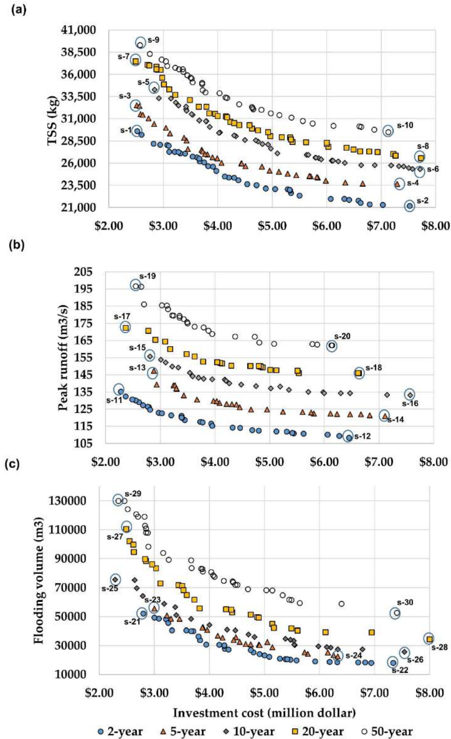
Figure 3.6. The non-dominated solutions obtained for different objectives (a) pollution load; (b) peak runoff; (c) flood volume. Two solutions were initially selected from each return period; the first solution corresponds to a very low objective reduction and minimum investment cost. The second solution corresponds to a very high investment cost and maximum objective reduction.
