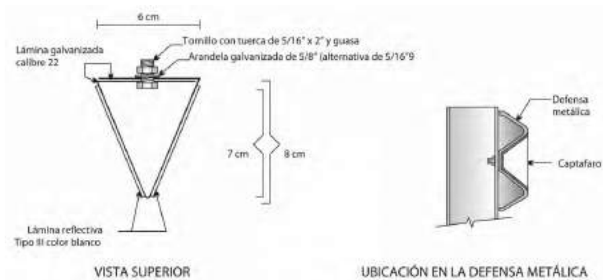
Figura 52. Captafaros
