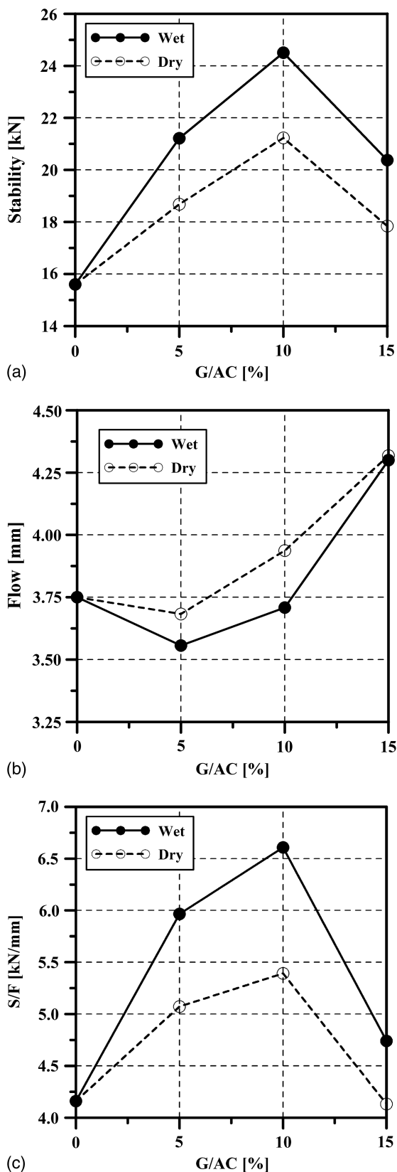
Fig. 3. (a) Evolution of stability S with G/AC ratio; (b) flow F with G/AC ratio; (c) S/F with G/AC ratio
