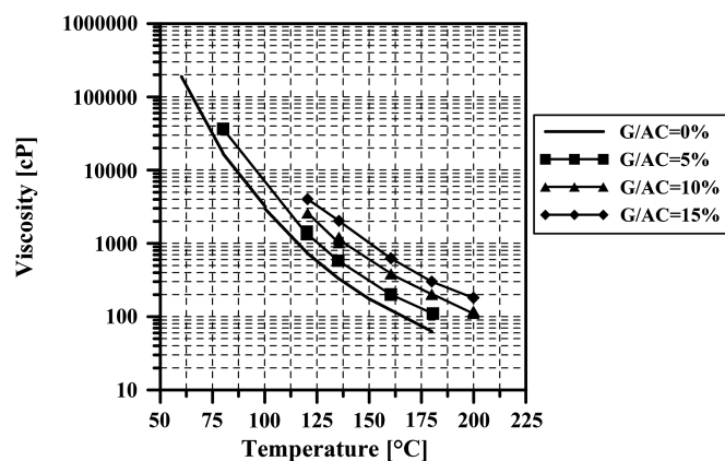
Fig. 2. Evolution of viscosity with temperature
