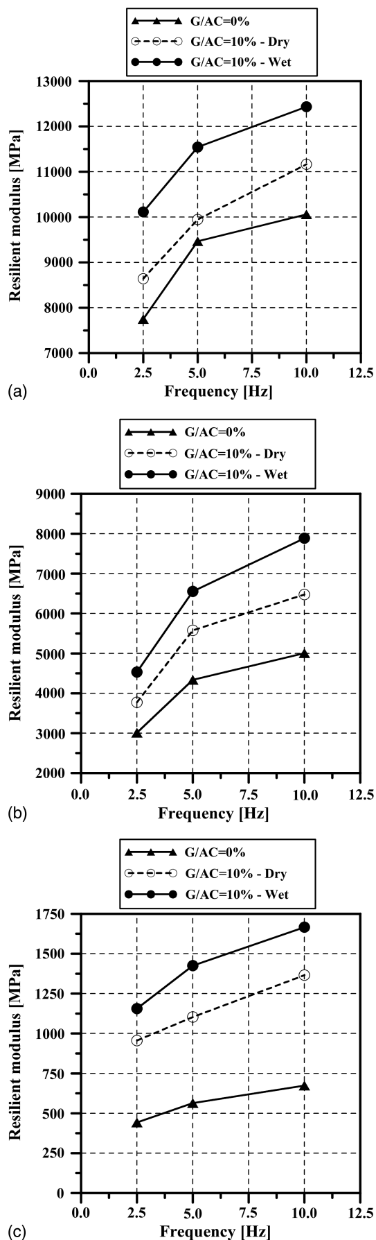
Fig. 7. Evolution of resilient modulus for (a) 10°C, (b) 20°C, and (c) 40°C
