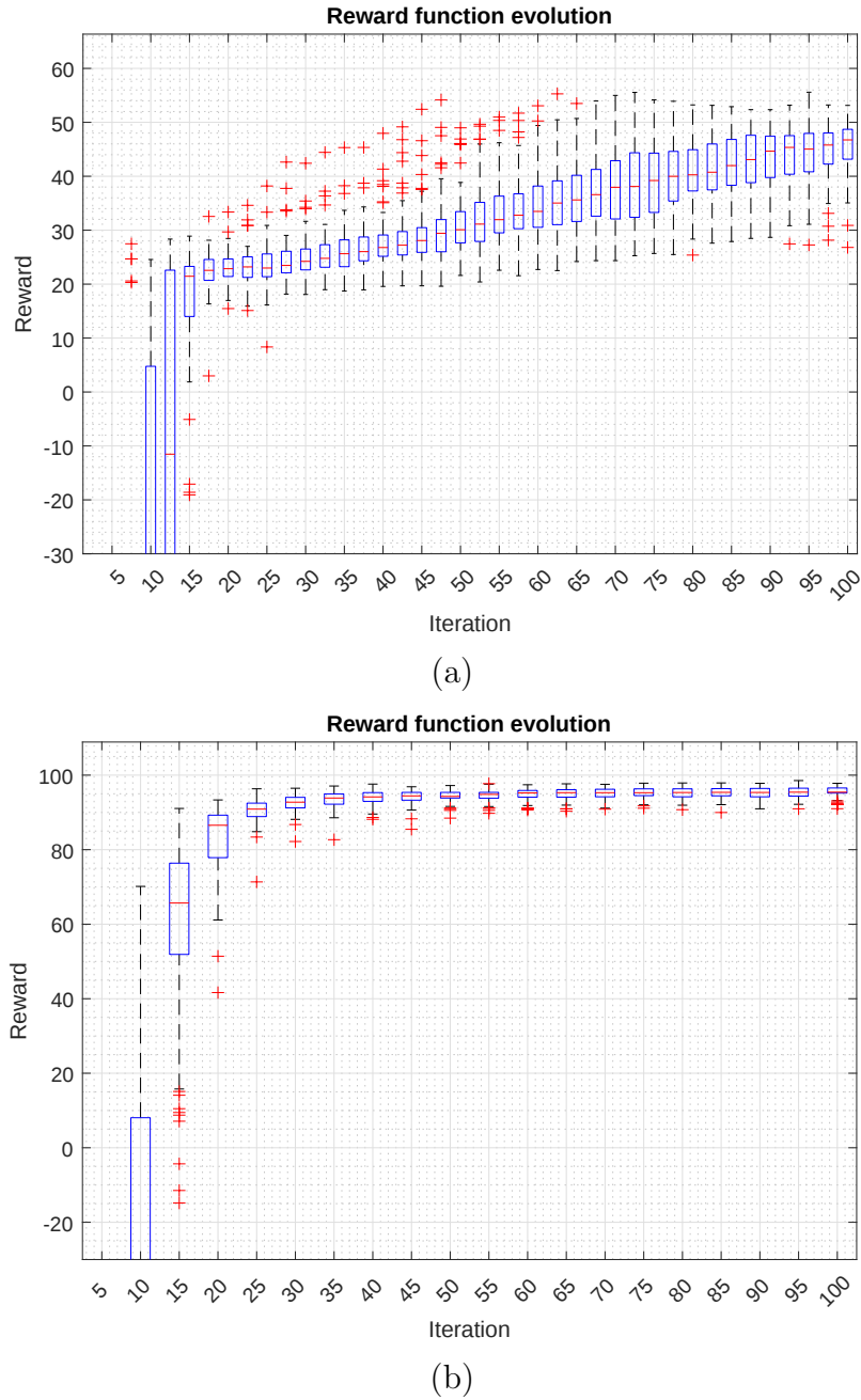
Figure 5-23.: Learning curves evolution - (a) Darwin-Mini (b) MAX-E2 - Concatenation of the boxplot diagrams for the reward at each iteration .
