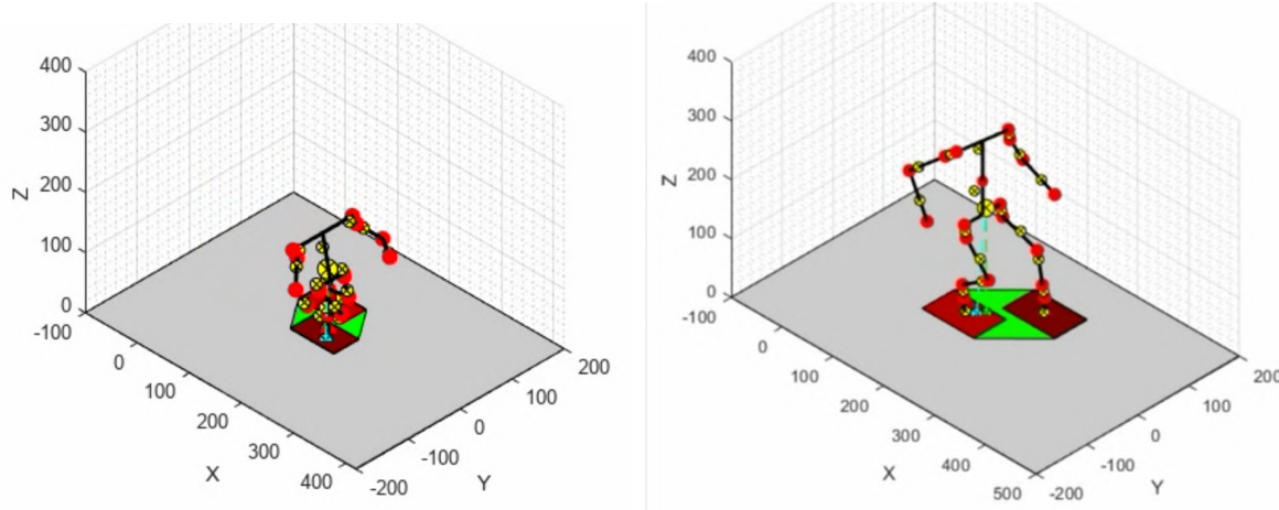
Figure 5-2.: Custom Simulator sample frames (Axis in millimeters) - (Left) Darwin Mini (Right) MAX-E2 - The red dots correspond to the position of the relevant frames of the robot, the small yellow dots correspond to the centers of mass of each link, and the larger yellow dot corresponds to the position of the entire robot CoM, the green dot corresponds to the projection of the CoM of the robot onto the ground, and the cyan dot corresponds to the ZMP.
