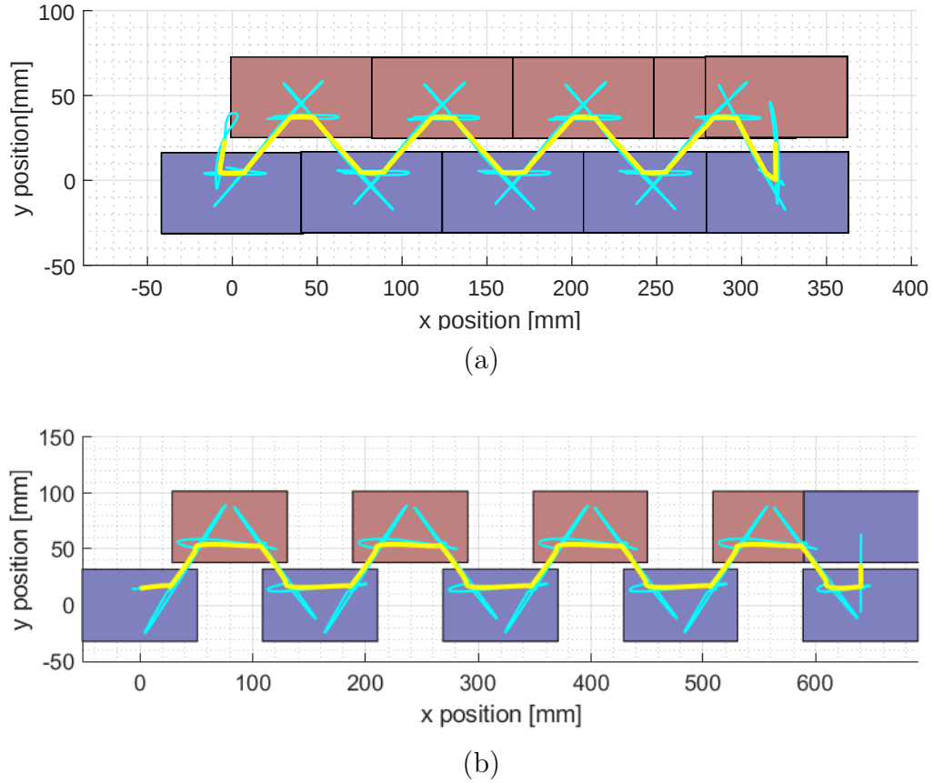
Figure 5-16.: ZMP behavior with Reinforcement Learning tuned Bézier trajectories - (a) Darwin Mini (b) MAX-E2 - The yellow line corresponds to the CoM trajectory, the cyan line shows the ZMP trajectory (mostly overlapped with the CoM), the blue rectangle corresponds to the position of the right foot, and the red rectangle corresponds to the position of the left foot.
