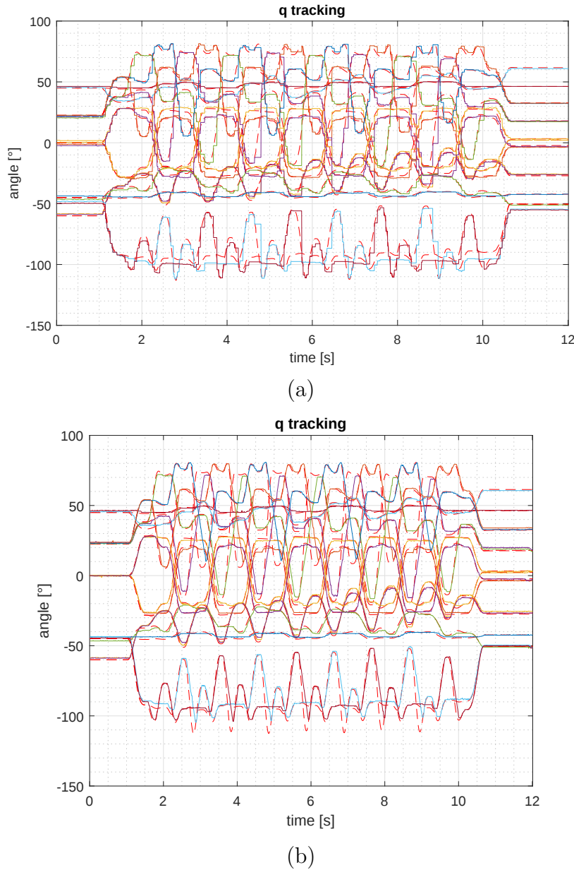
Figure 5-9.: Virtual and real joint behavior of the robots with manually tuned Bézier trajectories - (a) Darwin Mini (b) MAX-E2 - The color lines correspond to the real values of the joint trajectories, and the red dotted lines correspond to their corresponding references.
