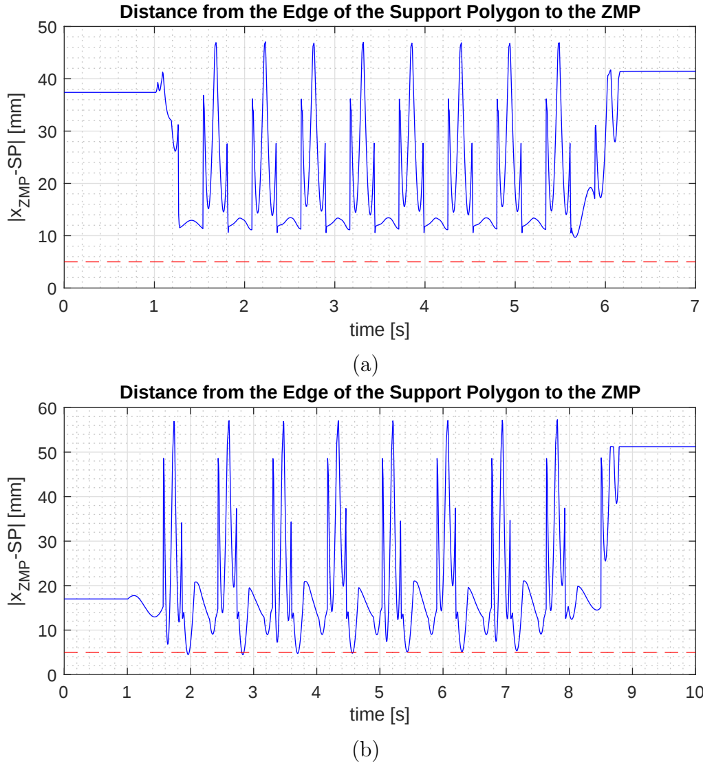
Figure 5-17.: Distance from the ZMP to the support polygon limit during gaits - (a) Darwin-Mini (b) MAX-E2 - the red dotted line corresponds to a safety boundary
