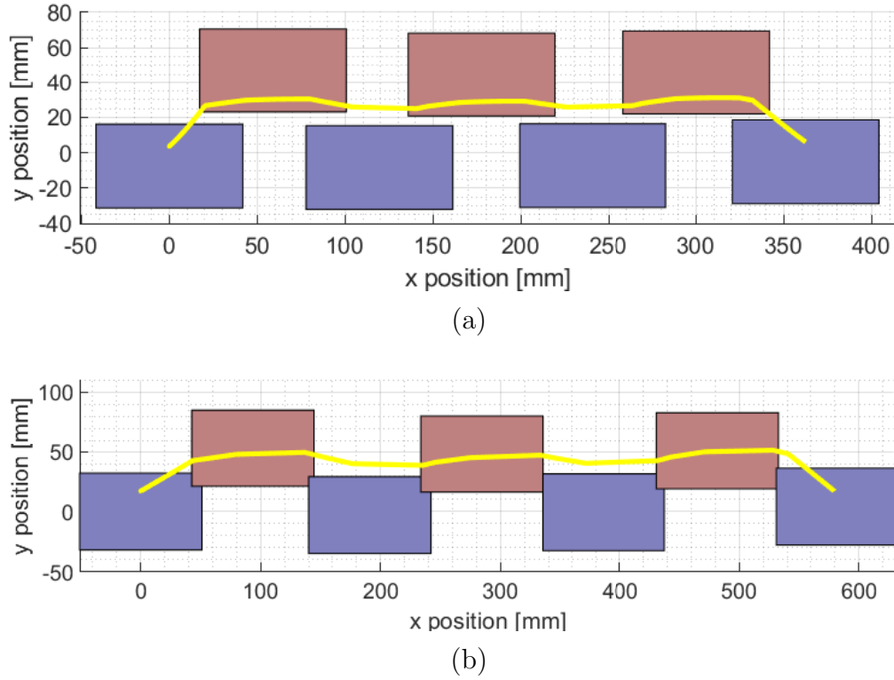
Figure 5-12.: Footprints and CoM behavior (before retargeting) - (a) Darwin-Mini (b) MAX-E2
