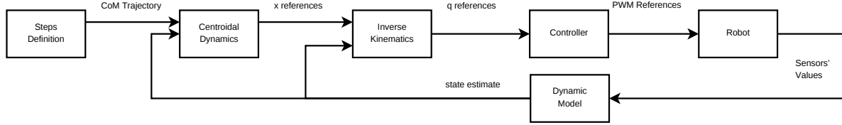
Figure 4-7.: Predefined gait control structure
