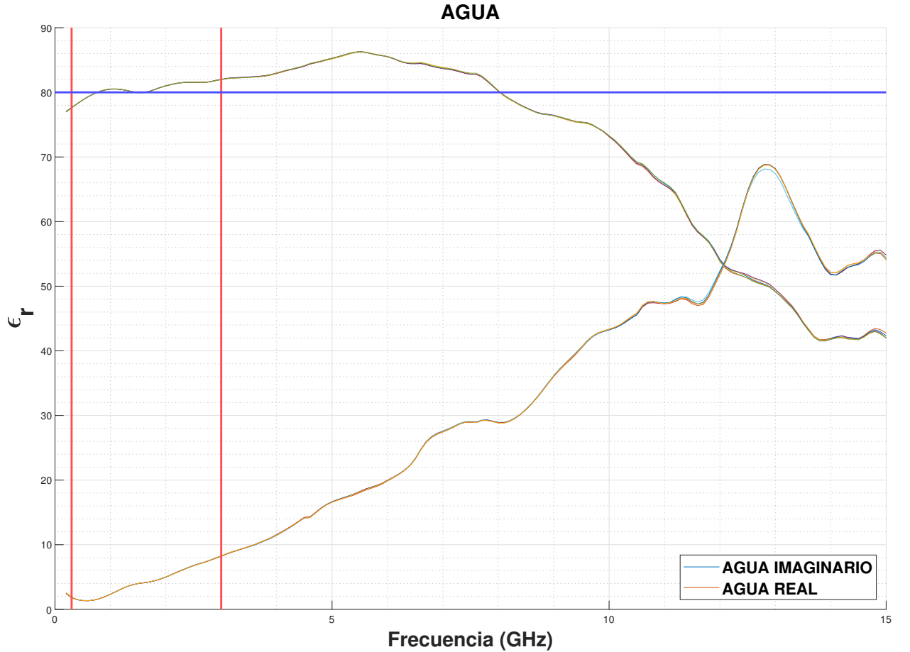
Figure 1.8: Measurement of electrical permittivity of water with Speag DAK 3.5 probe (manufactured by Speag) and Anritsu Master MS2028C vector network analyzer (VNA)
