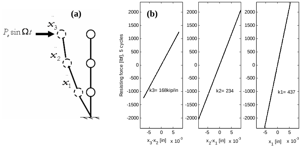
Figure 5: Story stiffness: (a) simple discrete model (b) hysteresis loops.
