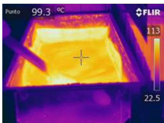
Figure 4. Thermal images within the thermal zone of the furnace during non-centrifuged cane sugar (NCS) processing: worker in the activity of stirring cane juice (A) and surface temperature of the cane juice in the evaporation process (B)
