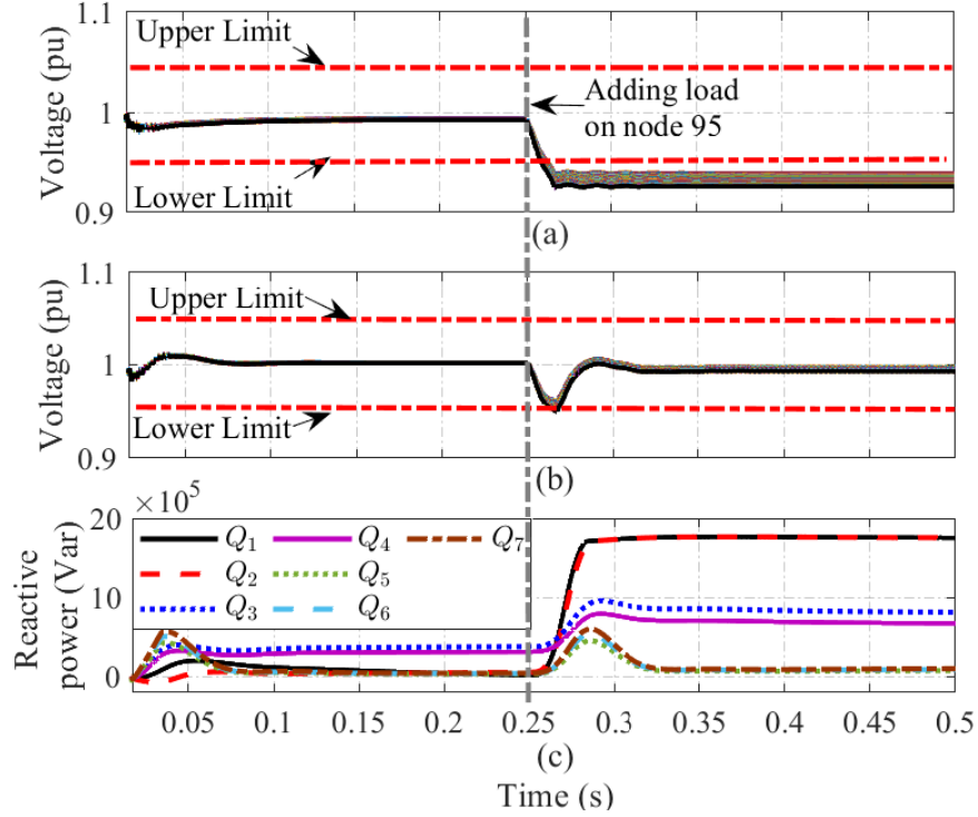
Figure 4.17: Dynamic voltage response in the 123-node distribution grid when the load is added at node 95. (a) In open-loop. (b) In closed-loop. (c) Reactive power injected by 7 parking lots (Scenario 4).
