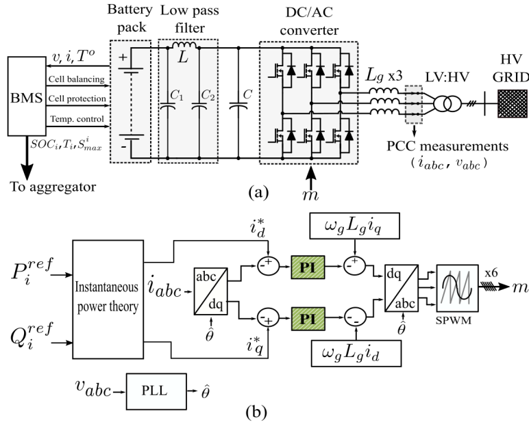
Figure 2.1: BESSs' diagram and its control architecture. (a) Topology. (b) PI controllers in dq0 reference frame.
