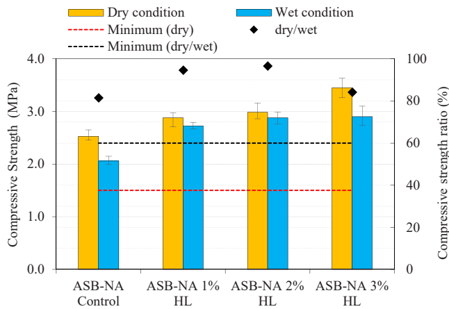
Fig. 10. Evolution of compressive strength with addition of HL.
