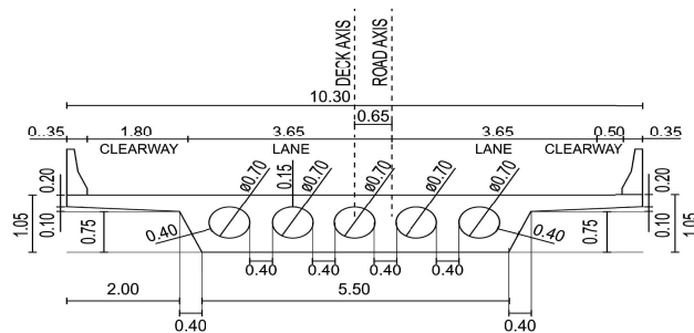
Figure 3. Cross section of the Portachuelo bridge. From: [13]
