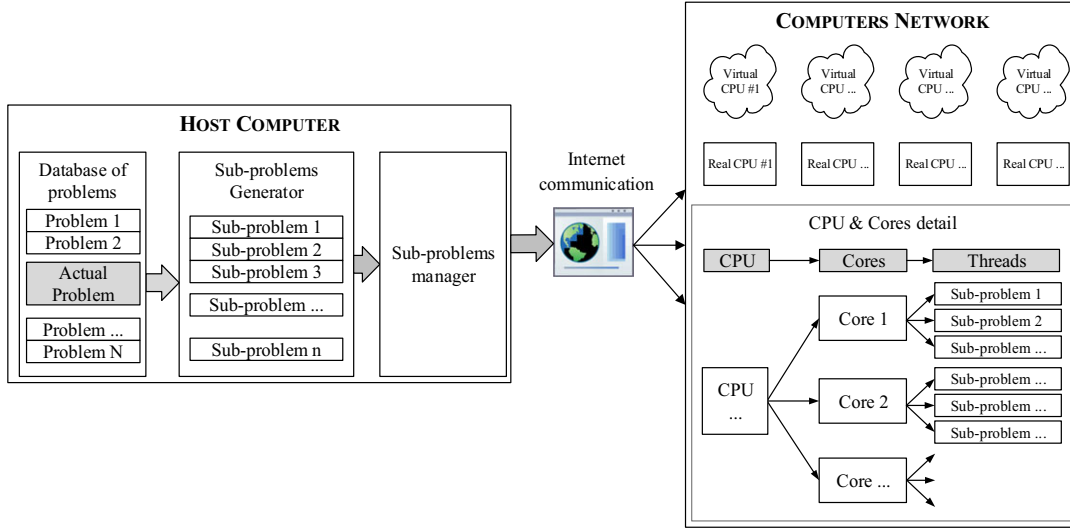
Fig. 1. Parallel processing.
