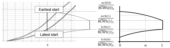
Fig. 6 Graphical interpretation of fuzzy \widetilde{BCWS}_t at period t
