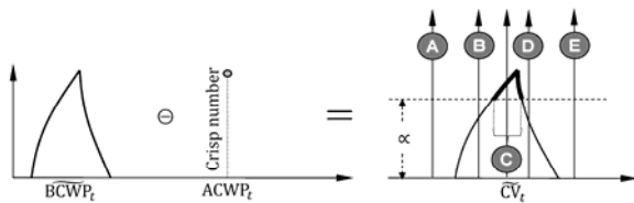
Fig. 8 Graphical interpretation of fuzzy cost variation
