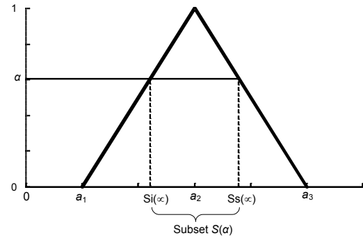
Fig. 3 \alpha -cut \tilde{A}(\alpha) of \tilde{A}
