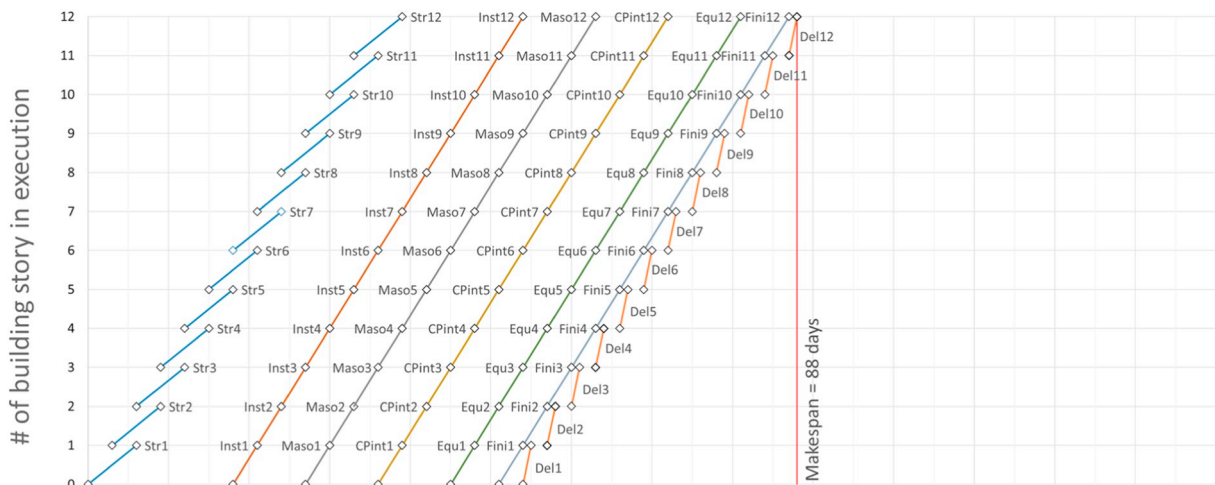
Fig. 9. Model 8 with multiple crews, non-accelerated routine, and non-continuity condition.
