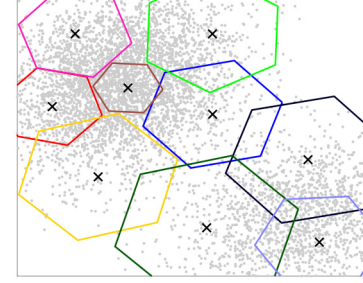
Fig. 14. Preferred MED solution with nine BTSs at the lower level is shown for the telecommunication problem. While the number of BTSs and their locations are determined by the UL, each BTS's strength and orientation are determined by the LL.
