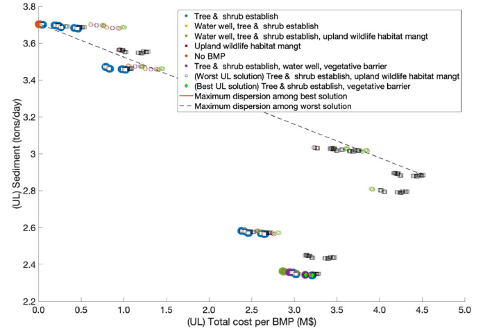
Fig. 9. UL solutions of the agricultural management problem, in which both objectives are minimized. Each colored circle corresponds to a different member of s_p^{\text{opt}} , and the best (spanning only from U.S. $3.13M to U.S. $3.21M cost) and worst (spanning widely from U.S. $0.03M to U.S. $4.52M cost) options in terms of expected deviation arising from LL solutions are marked with green diamonds and white squares, respectively. Dominated solutions are shown with transparent centers.
