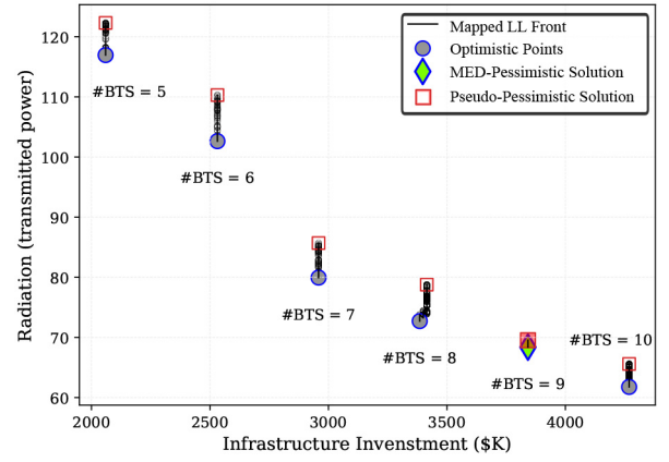
Fig. 12. Optimistic solutions in the UL-objective space for the telecommunication management problem. The B = 9 solution has the minimum MED and is the preferred solution.
