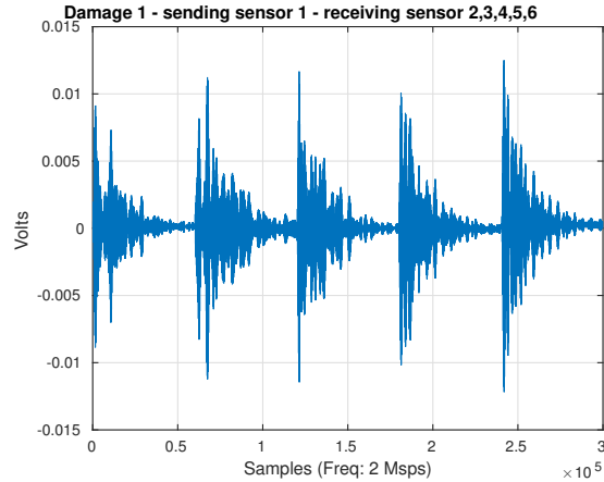
FIGURE 2.3: Received signals in the actuation phase 1 when damage 1 is performed to the structure.
