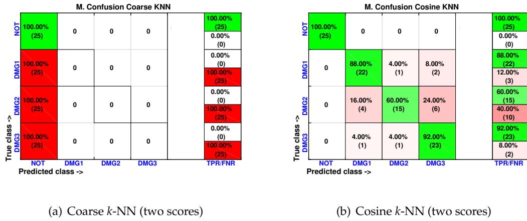
FIGURE 2.33: Confusion matrix using coarse k -NN (left) and cosine k -NN (right) when the feature vector is formed by the first two principal components.
