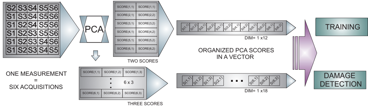
FIGURE 2.13: Feature vector organization.
