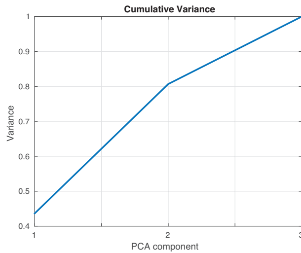
FIGURE 2.25: Cumulative contribution rate of variance accounted for the principal components from the data acquired from the aluminum plate.
