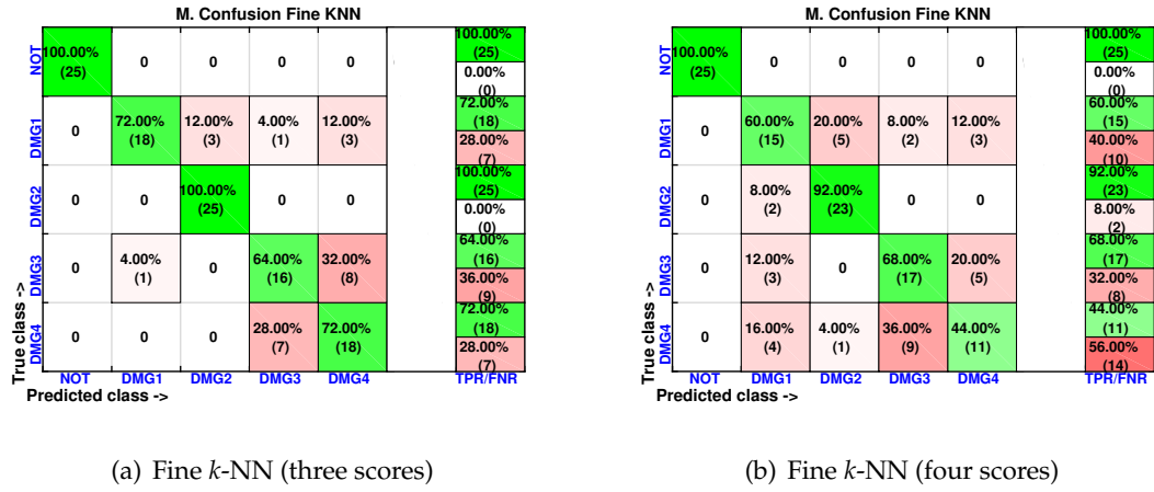
FIGURE 2.21: Confusion matrix using fine k -NN when the feature vector is formed by the first three principal component (left) or by the first four principal components (right).
