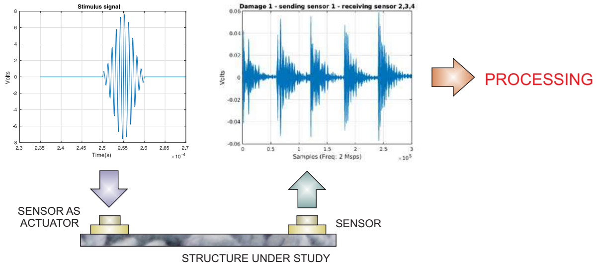
FIGURE 3.4: Signal excitation.
