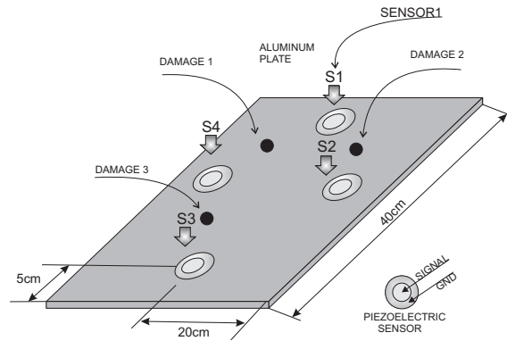
(a) Specimen 2. Aluminium plate schematic
