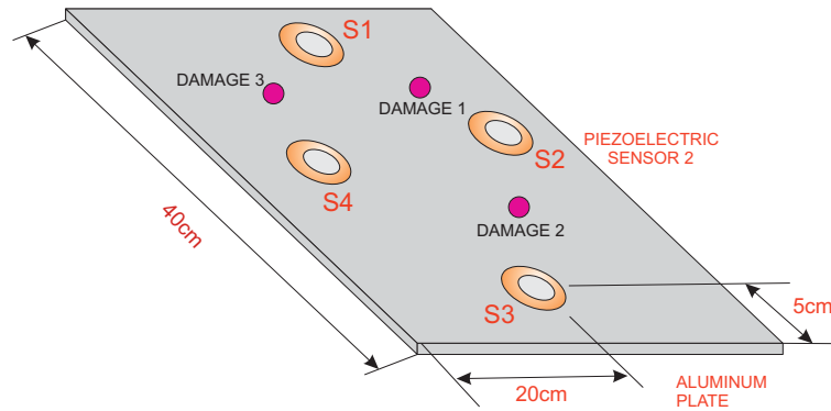
FIGURE 3.8: Aluminum plate instrumented with four piezoelectric sensors.
