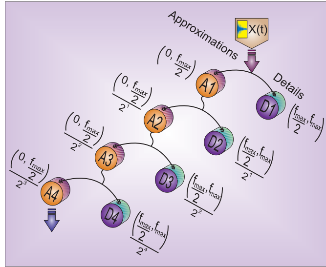
FIGURE 1.8: Wavelet decomposition
