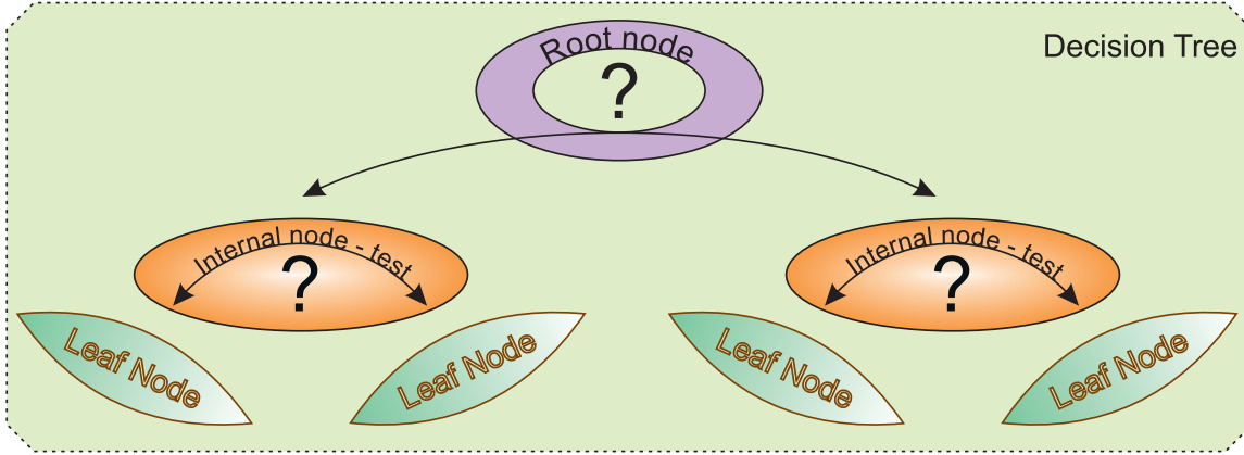
FIGURE 1.7: Desicion tree
