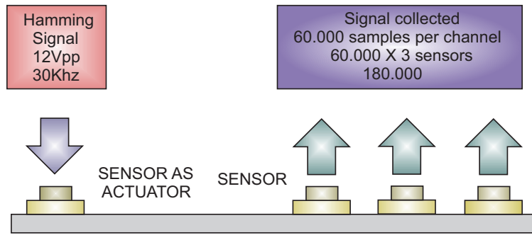
FIGURE 4.5: Structure exploration
