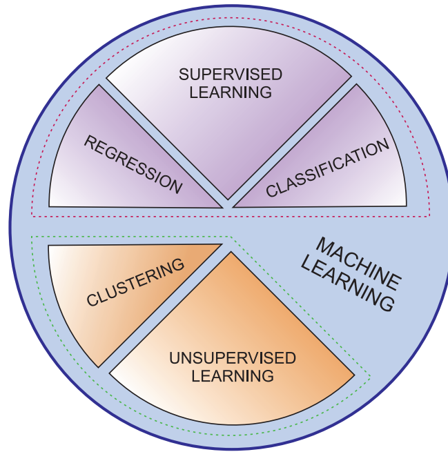
FIGURE 1.5: Machine Learning
