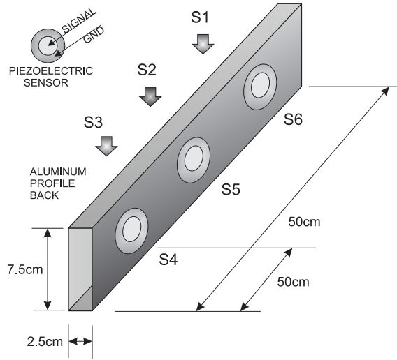
(a) Specimen 1. Aluminium profile schematic
