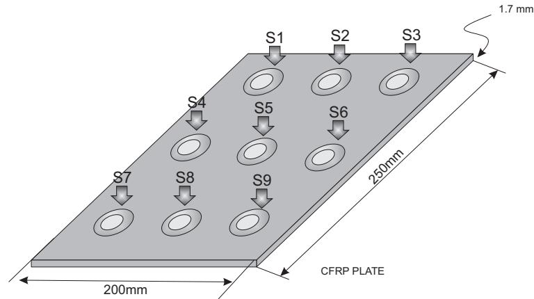
FIGURE 4.12: Specimen 2 - CFRP composite plate, sensors distribution.
