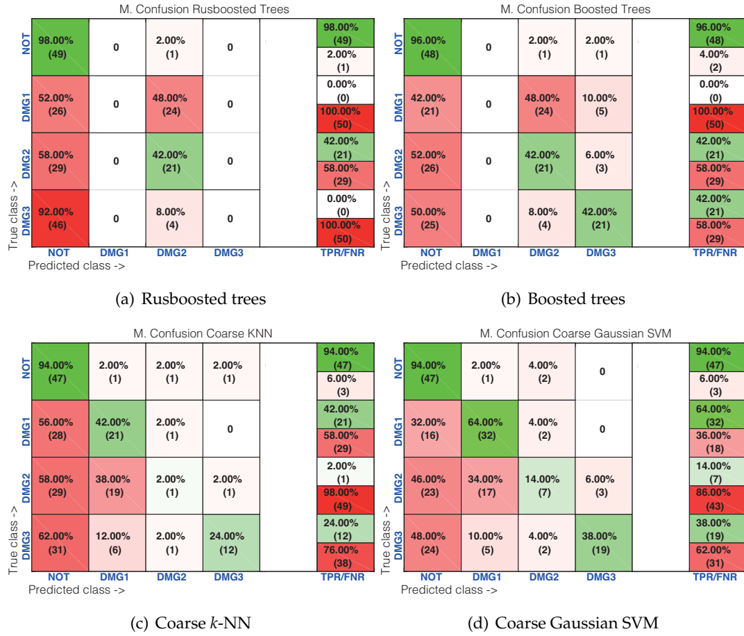
FIGURE 3.17: Confusion matrix using (a) rusboosted trees; (b) boosted trees; (c) coarse k-NN; and (d) coarse Gaussian SVM.
