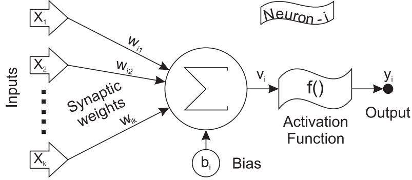
FIGURE 1.3: Neuron model
