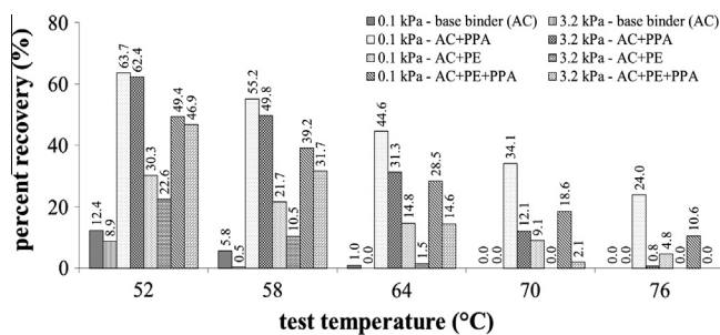
Fig. 2. Percent recoveries of asphalt binders.
