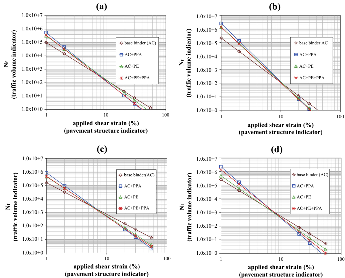
Fig. 1. Fatigue models from the VECD analysis: (a) short-term aging at 25 °C; (b) long-term aging at 25 °C; (c) short-term aging at 35 °C; (d) long-term aging at 35 °C.
