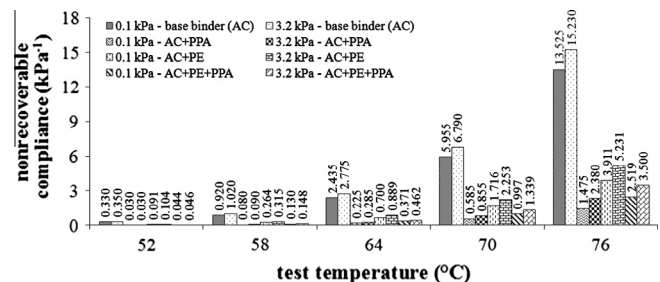
Fig. 3. Nonrecoverable compliances of asphalt binders.
