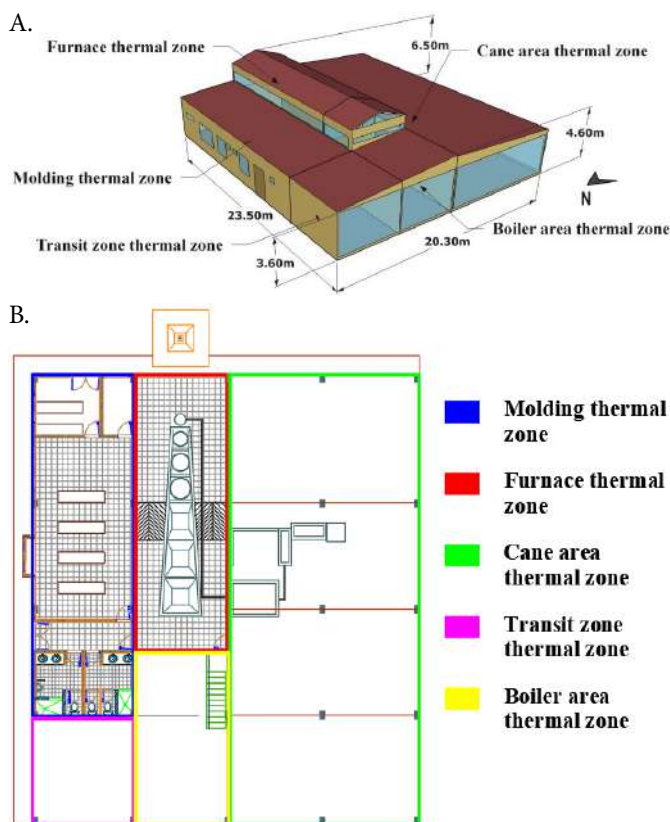
Figure 2. Facility for the preparation of NCS (A) and the geometry and thermal zones of the architectural plant (B)
