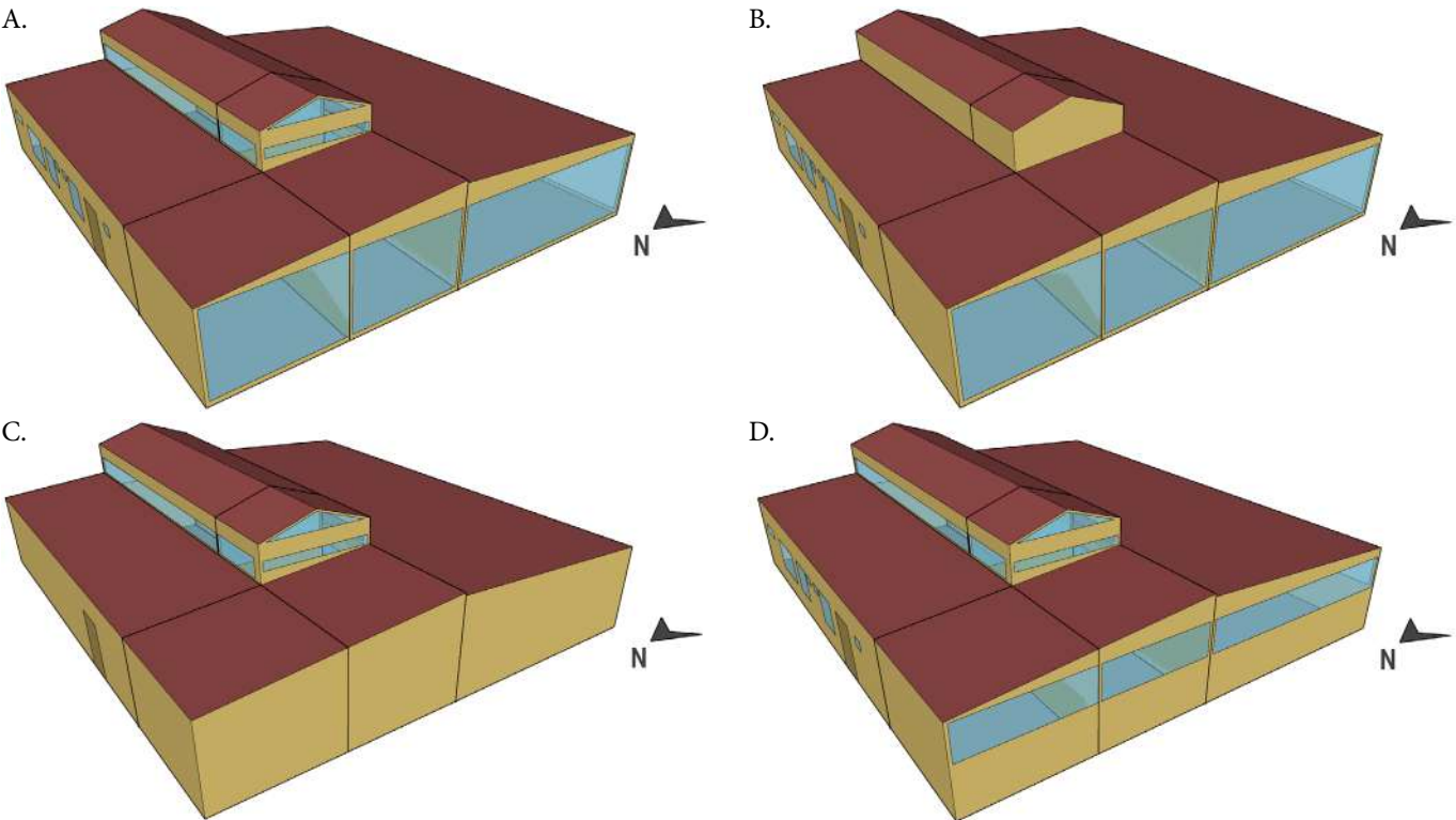
T1, T2, and T3 - Perimeter enclosure and lantern window open, with each covered in zinc, fiber cement, and clay ceramic, respectively; T4, T5, and T6 - Perimeter enclosure open and lantern window closed, with each covered in zinc, fiber cement, and clay ceramic, respectively; T7, T8, and T9 - Perimeter enclosure of solid brick, lantern window open, with each covered in zinc, fiber cement, and clay ceramic, respectively; and T10, T11, and T12 - Perimeter enclosure of perforated brick and lantern window open, with each covered in zinc, fiber cement, and clay ceramic, respectively
