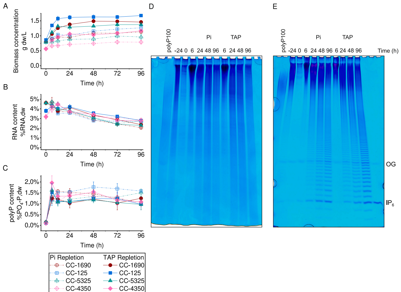
Fig. 4. PolyP reserves are rapidly resynthesized on provision of Pi after 24 h of Pi deprivation. OD 750nm = 1.0 cells were harvested (washed) and resuspended in TA media. After 24 h, the cultures were repleted to 1 mM Pi with either KPO 4 solution (dashed dotted lines) or resuspended in fresh TAP media (solid lines), and monitored for 96 h. A Biomass concentration (g dw/L), B RNA content in biomass (% RNA, dw), C. PolyP content in the biomass (% PO 4 -P, dw). D. 20 % and E 33 % representative PAGE of CC-1690 RNA volume equivalent to 500 µg dw. Wells from left to right: polyP100 loading control, -24 h (OD1.0 cells before Pi deprivation), 0 h (24 h Pi-depleted cells before Pi repletion), 6–96 h (After repletion with KPO 4 ), 6–96 h (After resuspension in TAP media) and 2 nmol of IP 6 standard. IP 6 overplus can be observed by increasing PAGE concentration to 33 % (E). OG; Orange G marker.
