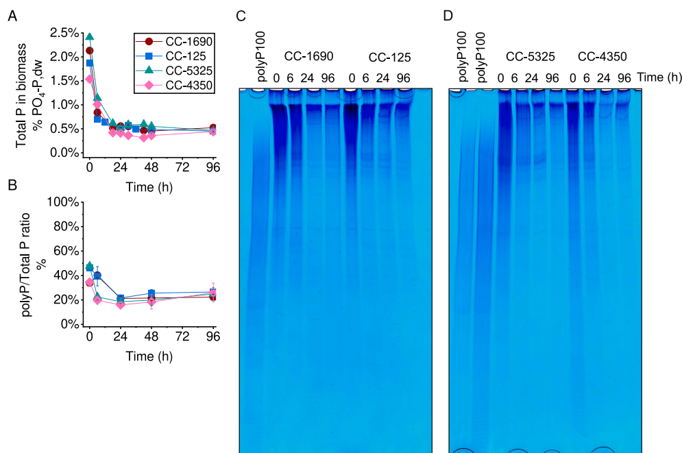
Fig. 3. The ratio of polyP to total P falls rapidly during Pi deprivation. A Total P content in biomass (% PO 4 -P, dw), B PolyP to total P mass ratio and C, D 20 % PAGE allows qualitative analysis of polyP. Left, polyP100 loading control, for the four strains of Chlamydomonas the RNA volume equivalent to 500 µg dw was loaded on each well for the 0, 6, 24 and 96 h time points after OD1.0 cells were harvested and resuspended in TA media.
