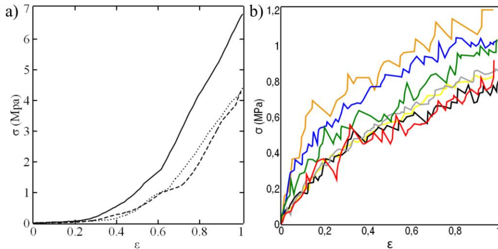
Figure 2. The strain stress curves: a) Pig Skin specimens and b) Latex Resistance Band specimens.
