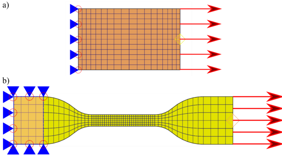
Figure 1. Boundary conditions in the numerical studies: a) Pig Skin and b) Latex Resistance Bands.
