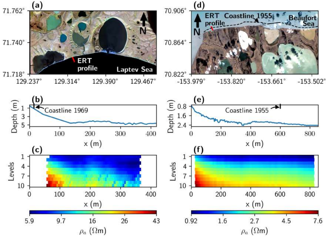
Fig. 3.1. Location and ERT data of our field studies. (a) Bykovsky field site located at the coast of the Laptev Sea in Northern Siberia (Sakha Republic, Russian Federation) and (d) Drew Point field site located at the coast of the Beaufort Sea in Northern Alaska (AK, United States of America), where the red lines indicate ERT profile locations and the black dashed line in panel (d) indicates the position of the 1955 coastline for Drew Point (Jones et al., 2008). (b) The recorded bathymetric profile along the ERT profile for Bykovsky and (e) for Drew Point indicating the 1969 (Schirrmeister et al., 2018) and 1955 coastline positions, respectively. The current coast position for both profiles is at x \approx -10 m. (c) Pseudosection of the recorded raw ERT data for Bykovsky, and (f) for Drew Point. Satellite image Bykovsky: Worldview3 satellite product from September 2 nd , 2016; copyright Digital Globe. Satellite image Drew Point: Planet satellite image from September 3 rd , 2017.
