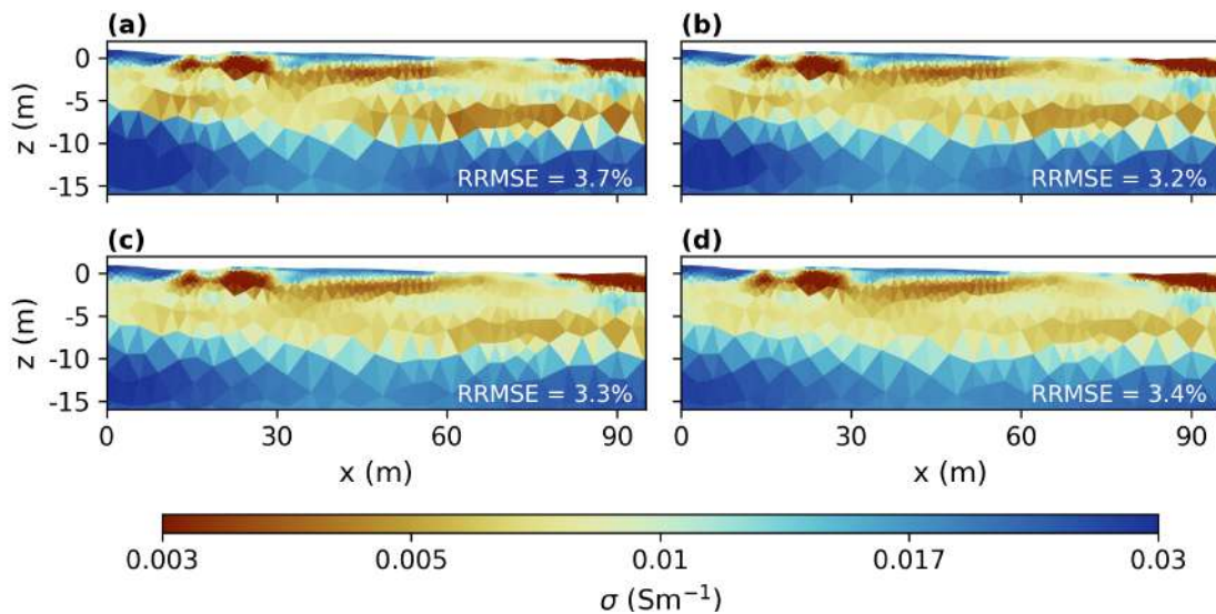
Fig. 4.4. Inverted electrical conductivity models of profile ERT2 considering different horizontal ( Cx ) and vertical ( Cz ) correlation lengths for geostatistical regularisation during data inversion. (a) Cx = 10 m and Cz = 1 m, (b) Cx = 20 m and Cz = 2 m, (c) Cx = 30 m and Cz = 3 m, and (d) Cx = 40 m and Cz = 4 m.
