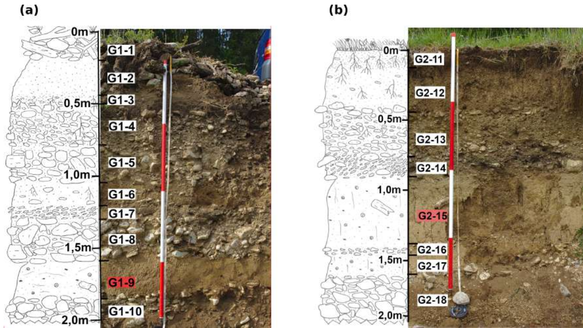
Fig. 4.9. Stratigraphic sections of the Grimbach alluvial fan from Schönleber et al. (2022). (a) profile G1 and (b) G2 with the locations indicated in Fig. 4.1d. The units G1-9 and G2-15 highlighted in red were sampled for radiocarbon dating.
