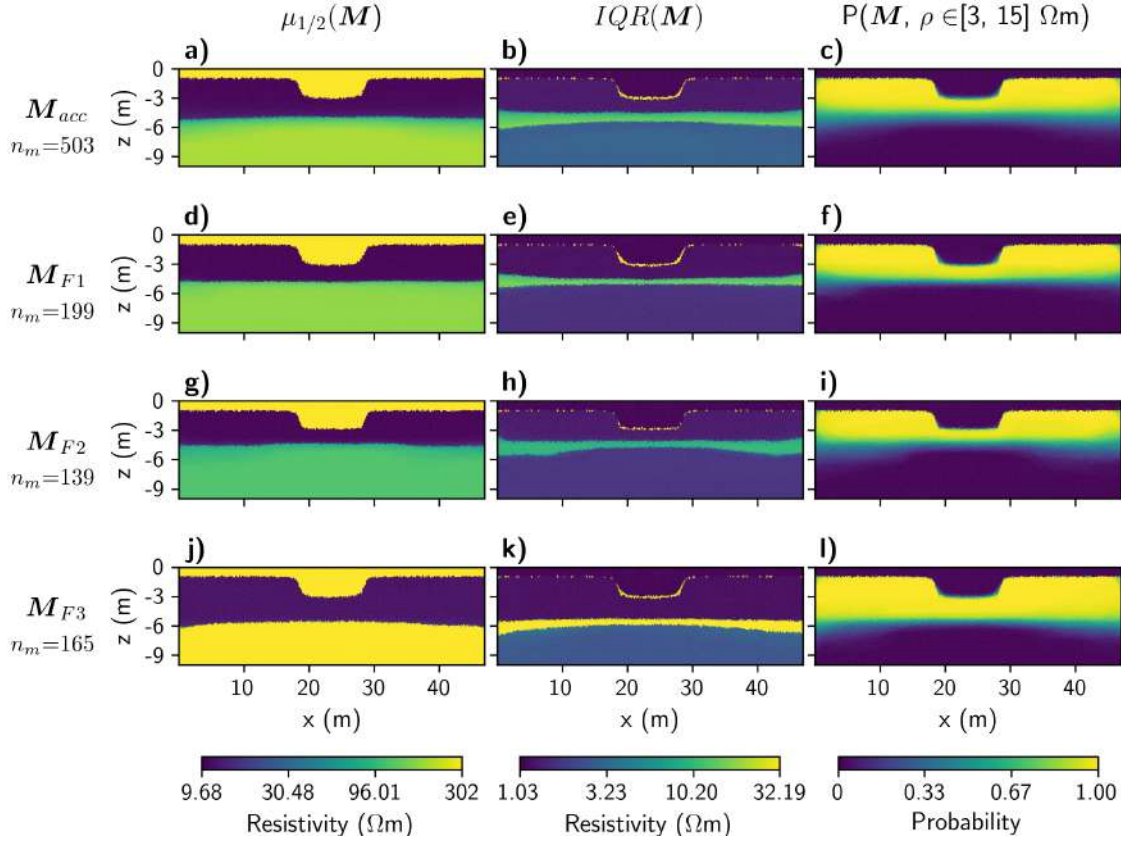
Fig. 2.4. Representation of the pixel-wise calculation of the \mu_{1/2}(M) , IQR(M) , and P(\rho \in [3, 15] \Omega\text{m}) for our synthetic example. (a-c) statistics for the accepted models M_{acc} and (d-l) for the clustered families M_{F1} , M_{F2} , and M_{F3} . n_m represents the size of each ensemble of models.
