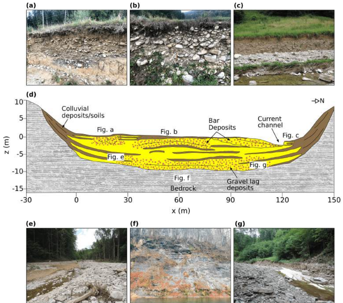
Fig. 4.10. Sedimentary architecture of the Grimm bach fan. (a) Channel fill structure found ~ 500 m upstream of the Grimm bach-Kocher confluence. (b) Detail of the interpreted bar deposit of Fig. 4.8b. (c) Colluvial deposits are overlying channel-bed deposits ~ 570 m upstream from the Grimm bach-Kocher confluence. (d) Inferred and idealised fan stratigraphy considering profiles ERT2, EMI1, GPR3, and available outcrops, where x = 0 m corresponds to the origin of the ERT2 profile and x = 95 m to its end. (e) Deposits of the last flood overlay a layer composed of fine materials in the middle reach of the Grimm bach (1-2 km upstream from our field site). (f) Outcrop of the bedrock on the left flank of the Kocher opposite the Grimm bach outlet. (g) Coarse material in the left flank and fine material to the right flank overlying bedrock in the upper reach of the Grimm bach (3-4 km upstream from our field site).
