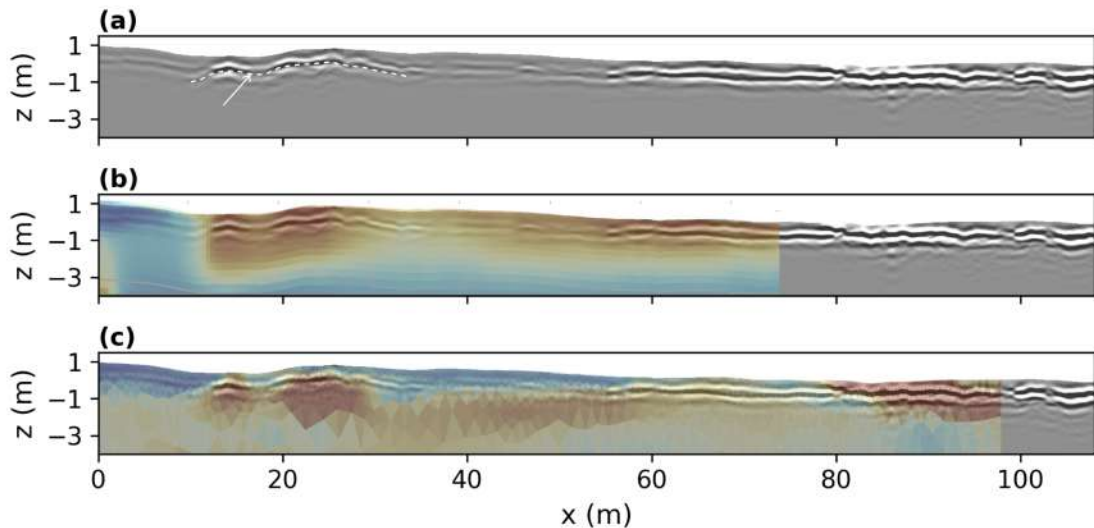
Fig. 4.7. Comparing GPR with electrical conductivity responses. (a) GPR3 profile overlying (b) EMI1 and (c) ERT2 models. The white dashed line in panel (a) indicates a general concave-down structure with a little concave-up structure marked by the white arrow. In panels (b) and (c), we use the same colour map as in Fig. 4.3a and Fig. 4.5b.
