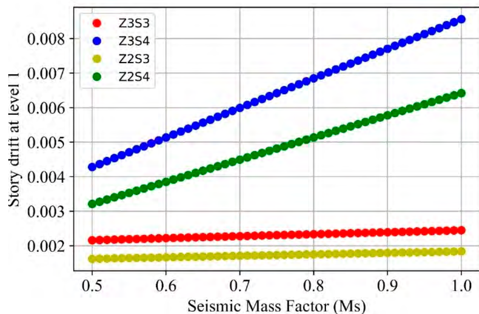
Figure 16. Variation of seismic mass factor (Ms) vs. drift at level 1.
