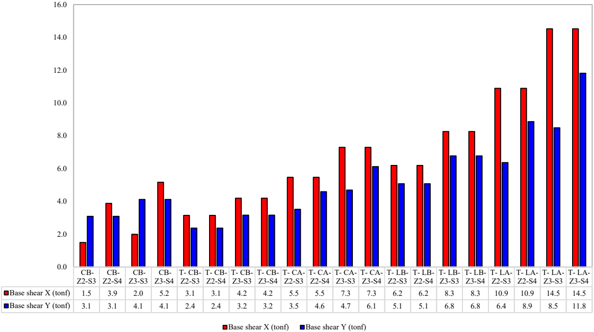
Figure 5. Base shear by direction.
