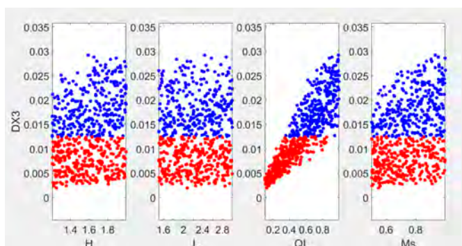
Drift X – level 3
