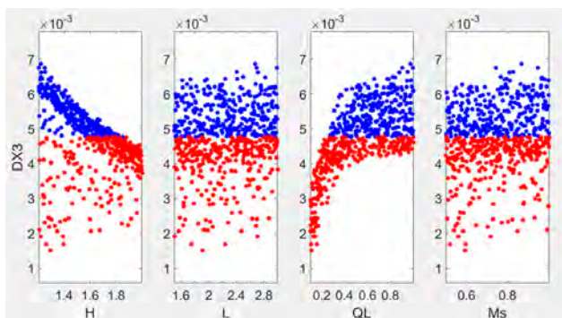
Drift X – level 3
