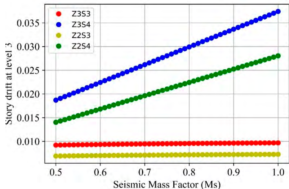
Figure 18. Variation of seismic mass factor ( M_s ) vs. drift at level 3.
