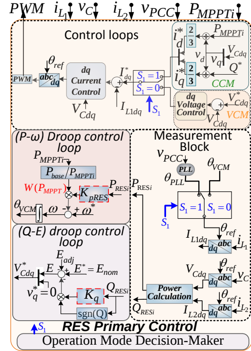
Fig. 13: Scheme of the Primary control for RESs.
