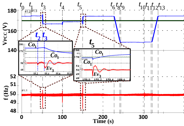
Fig. 20: Common Bus Voltage and Frequency.
