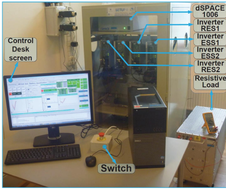
Fig. 18: Experimental Setup at the laboratory.
