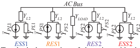
Fig. 3: Topological operation of the microgrid when all the DERs operate in CCM.
