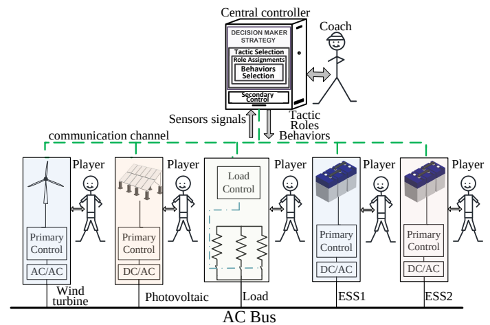
Fig. 6: Overall control architecture.
