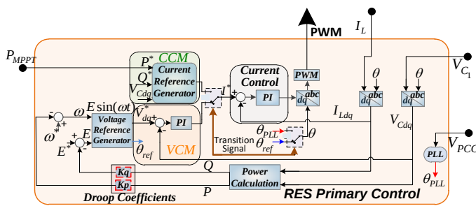
Fig. 4: Control Diagram of the RESs.
