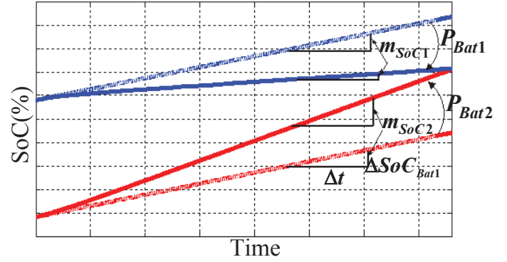
Fig. 3: Expected behaviour for the equalization of SoCs.
