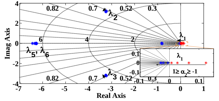
Fig. 9: Root locus plot of the microgrid under adjustment of weighting factors \alpha_i .
