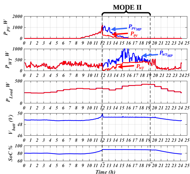
Figure 6. Operation of the microgrid for time period of 24h.
