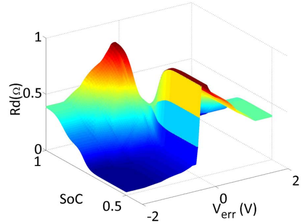
Fig. 8. Control surface of the fuzzy inference system.
