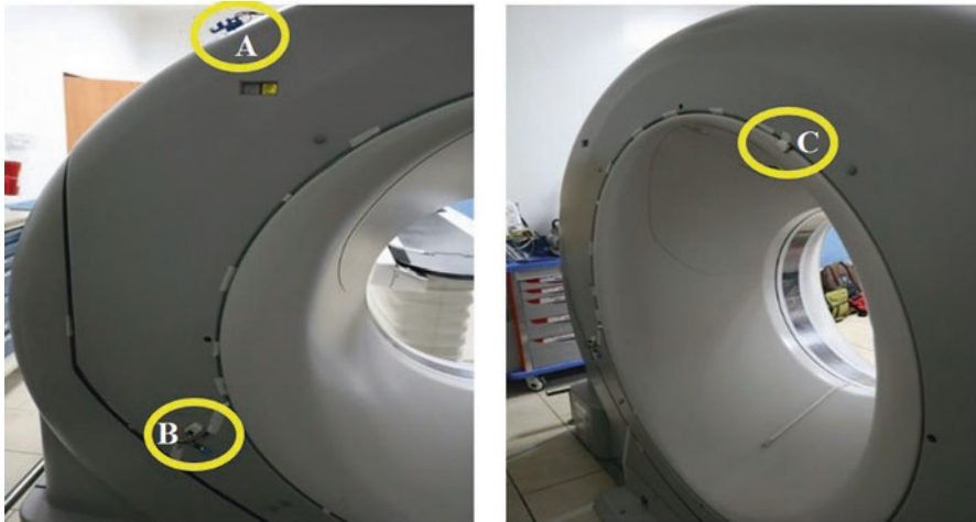
Fig. 6 Installation of the sensors; (a) sound sensor, (b) temperature and humidity sensor, (c) vibration sensor
