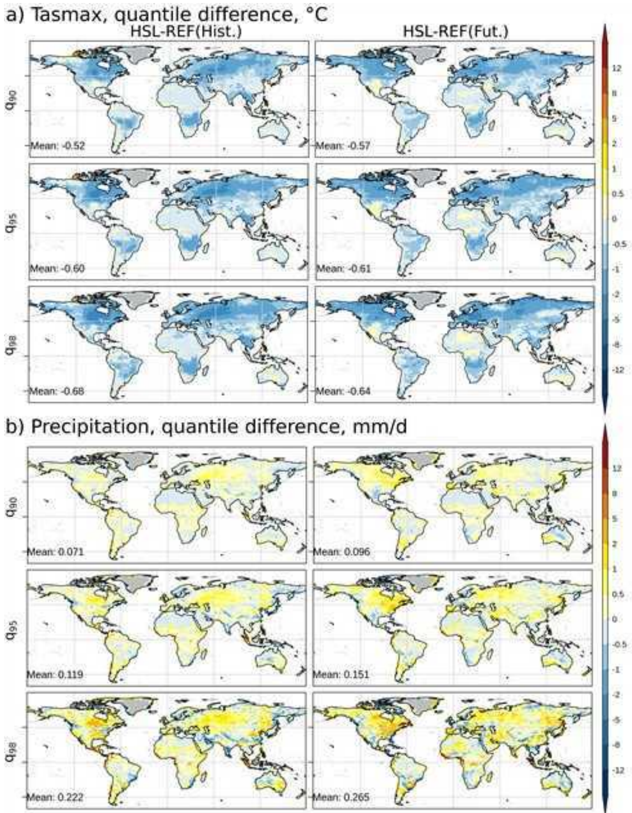
Figure 3.12: Difference of quantiles for historical (1980-2010, first column) and future (2070-2010, second column) period, between HSL and REF simulations, for maximum air temperature Tasmax (a) and precipitation P (b).
