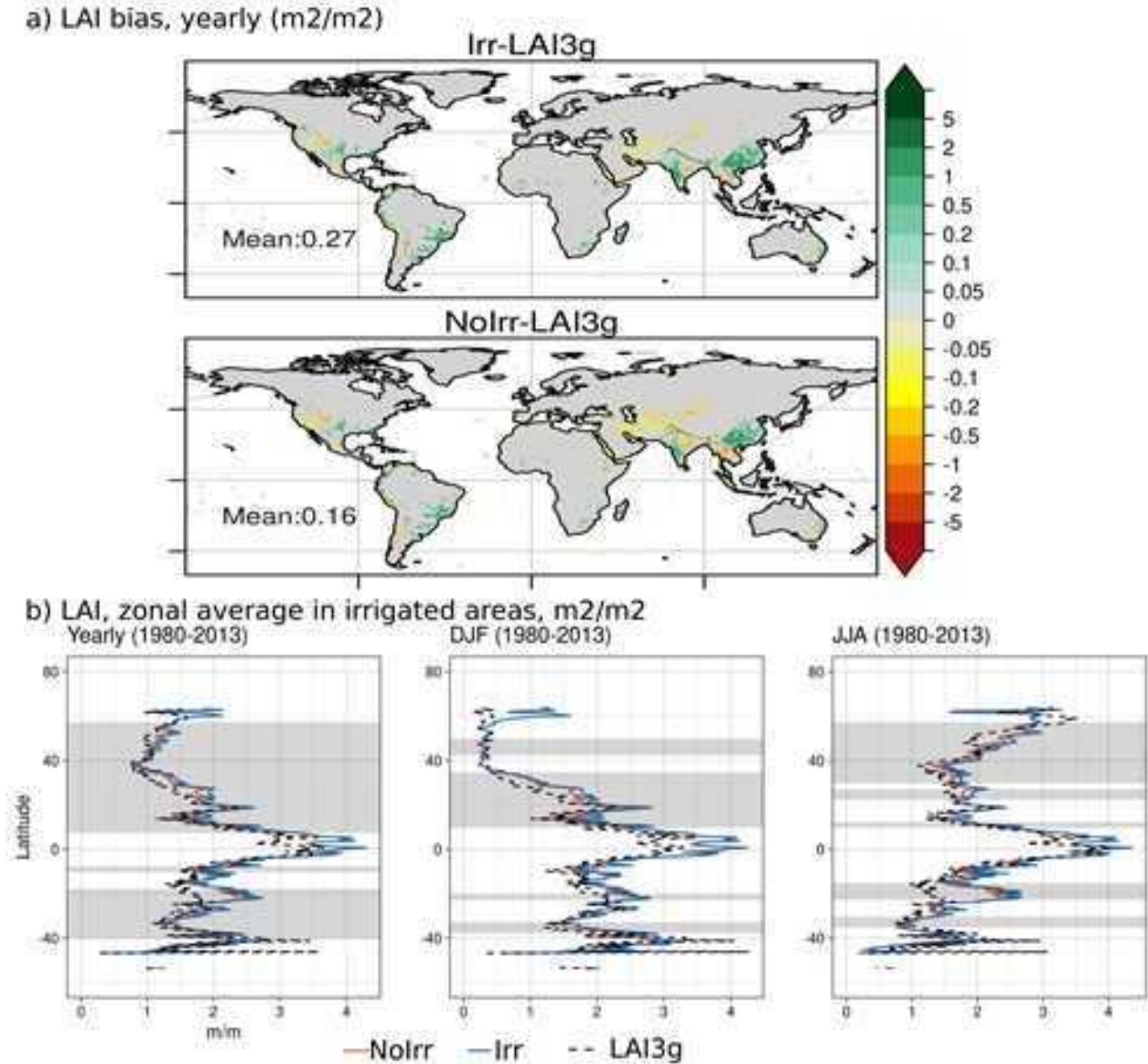
Figure 4.11: Difference of yearly average values for 1980 - 2013 between NoIrr and Irr simulations, and LAI3g (a) for LAI in m^2/m^2 . Statistical significance of the mean differences is tested at each point with a Student's test ( p = 0.05 ). The areas with insignificant changes or no irrigated fraction are left gray. Zonal average values of areas with irrigated fractions for yearly, boreal summer (JJA) and boreal winter (DJF) of LAI for period 1980 - 2013 (b) in m^2/m^2 . Gray areas for zonal average values depict the latitudes with significant differences between Irr and NoIrr simulation, according to the t-student test ( p = 0.05 ).
