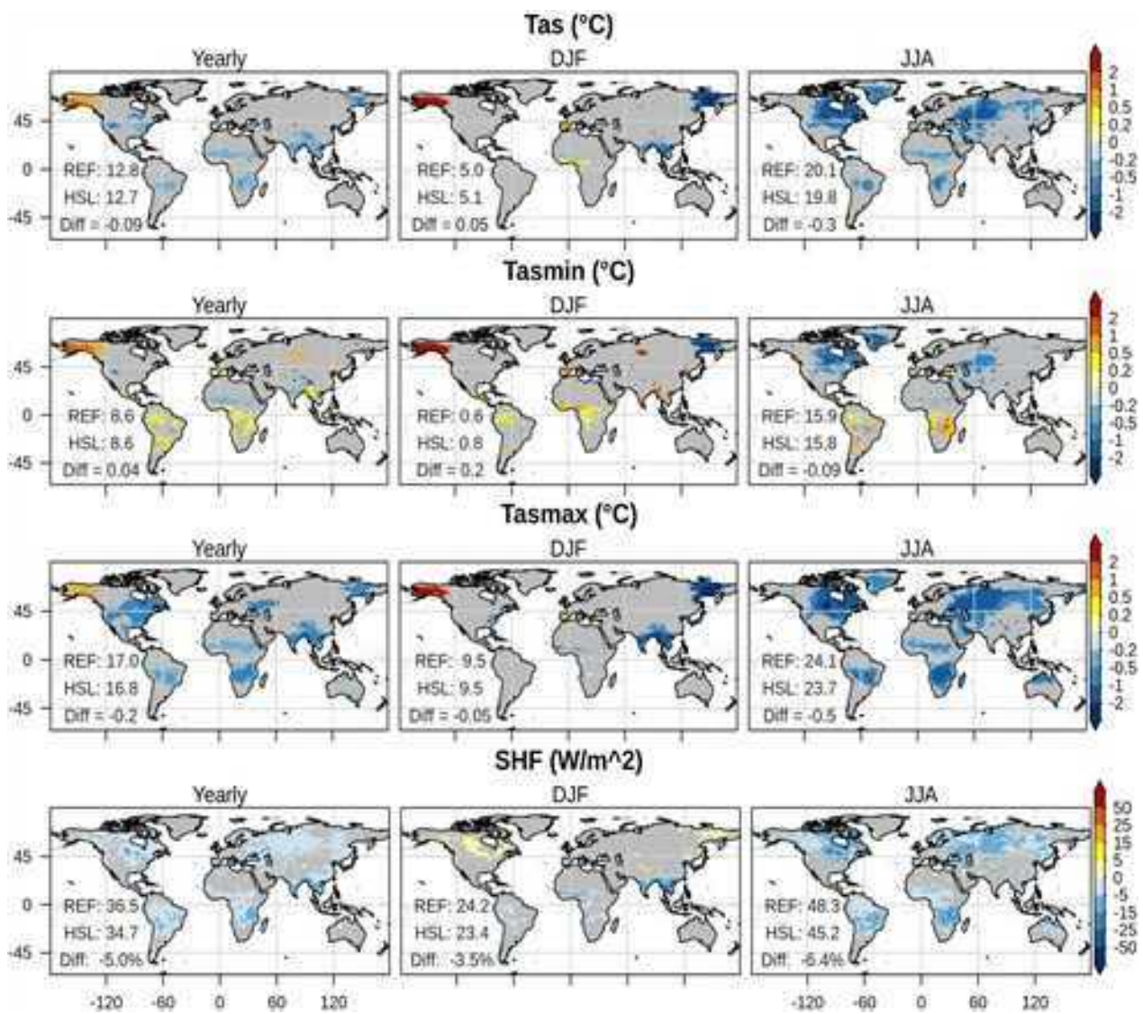
Figure A.2: Same as Figure A.1 but for Tas, Tasmin, Tasmax, and SHF.
