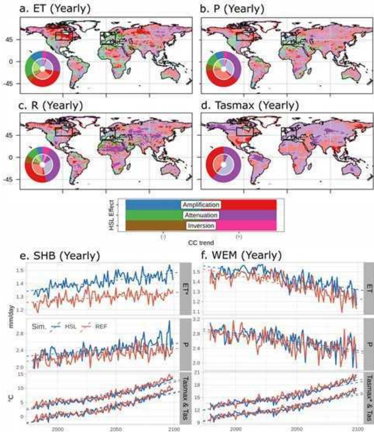
Figure 3.6: Spatial distribution of hillslope flow modulation in yearly mean values for period 1980–2100, ET (a), P (b), R (c) and Tasmax (d). The areas with insignificant changes in hillslope flow modulation have transparent colors. Doughnuts show the distribution of hillslope flow modulation (outer circle) and the corresponding partitioning of the significant & insignificant modulation (inner circle). We use a Mann-Kendall test ( p = 0.05 ). The table below the maps define the modulation types and corresponding colors. Regional annual average values of ET, P, and Tas & Tasmax in Southern Hudson Bay, SHB (e) and Western Europe and the Mediterranean, WEM (f) for 1980–2100. Statistical significance of the modulation was tested with a Mann-Kendall test ( p = 0.05 ), and significant trends are shown by a * in the vertical titles. In the Tasmax & Tas panel, the top blue and red lines correspond to Tasmax.
