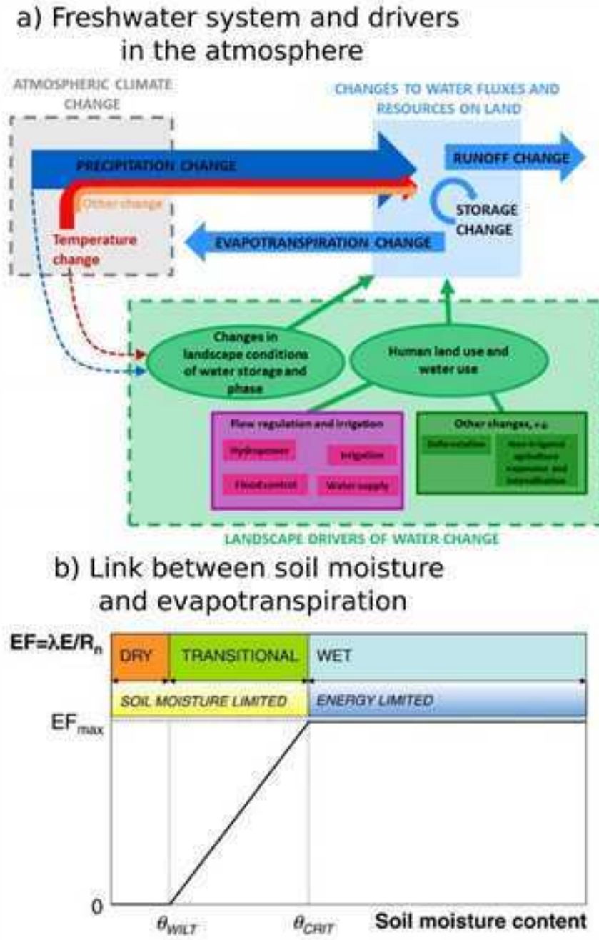
Figure 1.3: Changes on freshwater system and possible drivers in the atmosphere (a), taken from Jaramillo and Destouni, 2015. Link between soil humidity regimes and evapotranspiration regimes according to the conceptual framework from Budyko (b), taken from Seneviratne et al., 2010. \theta_{wilt} and \theta_{crit} are respectively the wilting point, and the critical soil moisture that constrains evapotranspiration, EF refers to the evaporative fraction from total rainfall, \lambda is the heat of vaporization, E is the evaporation mass, and R_n is the net radiation.
