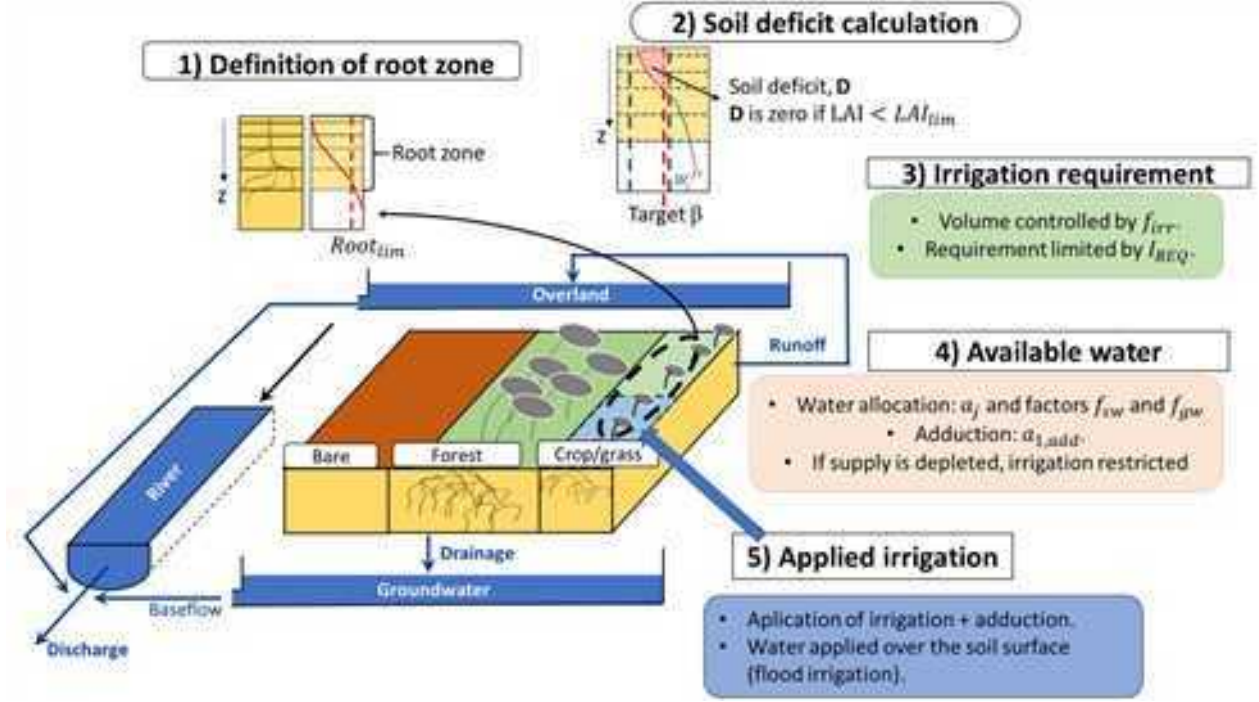
Figure 4.1: ORCHIDEE model and new irrigation scheme. See text for explanation of parameters
