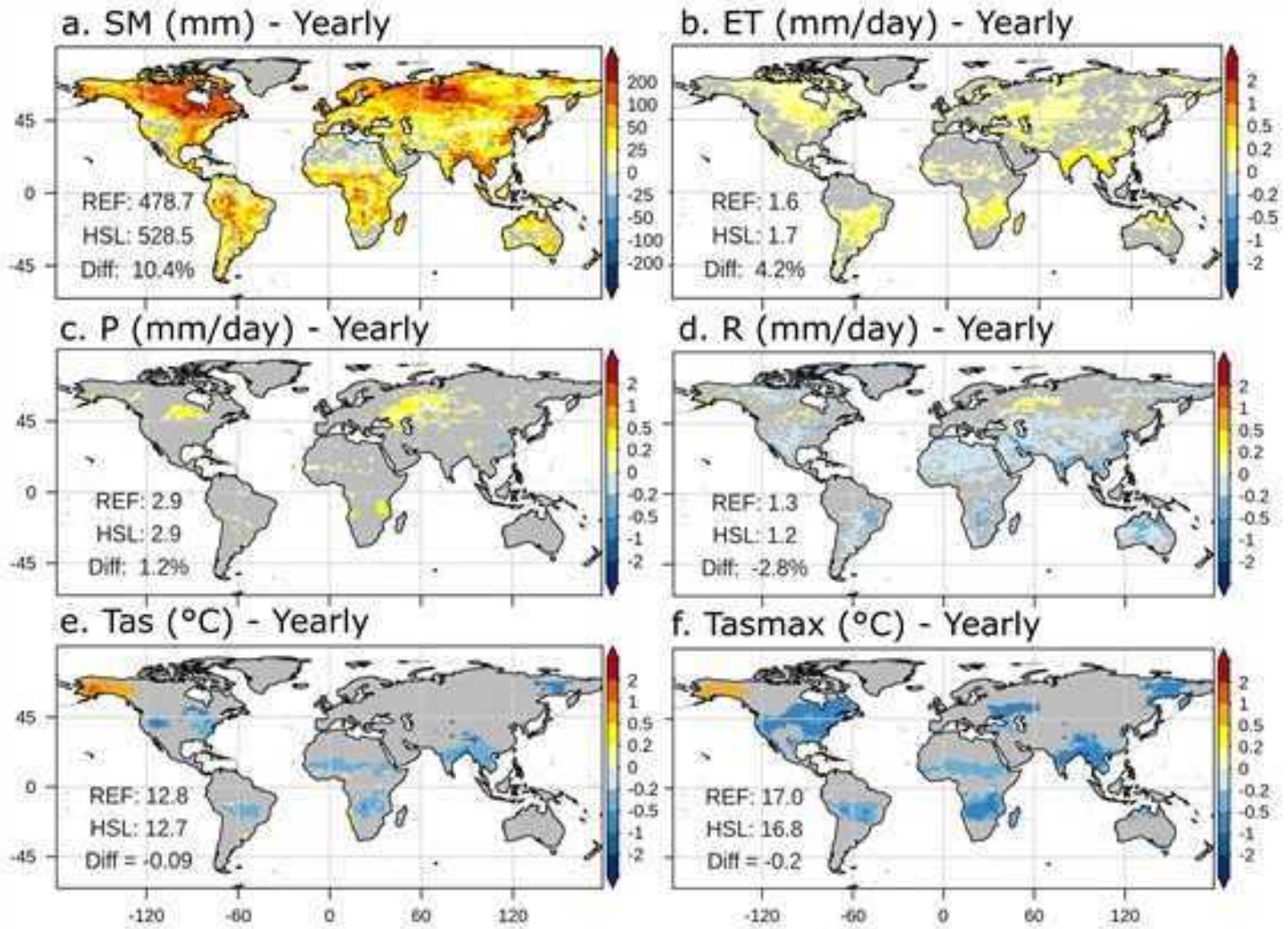
Figure 3.2: Change in mean yearly values between HSL and REF for the period 1980–2010: (a) SM, (b) ET, (c) P, (d) R, (e) Tas, (f) Tasmax. Statistical significance of the mean differences is tested at each point with a Student test ( p = 0.05 ). The areas with insignificant changes are left gray.
