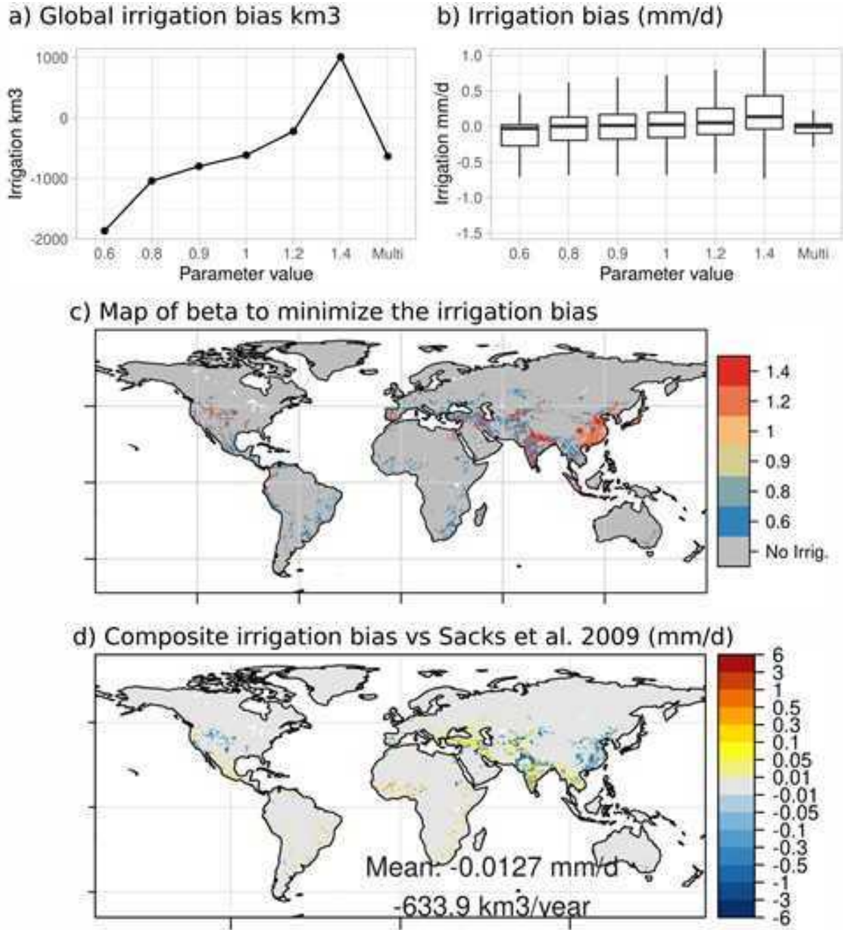
Figure 4.3: Calibration of \beta value with Sacks et al., 2009 dataset as observed value, using outputs from the short simulations. Calibration of \beta value using global irrigation volumes in \text{km}^3 (a) and boxplot using grid-cell bias in \text{mm/d} (b). Map of \beta to minimize the irrigation bias, according to the short simulations (c) and composite map of irrigation bias according to the calibrated \beta value in \text{mm/d} (d). Multi simulation in a) and b) correspond to the bias of the composite map shown in (d).
