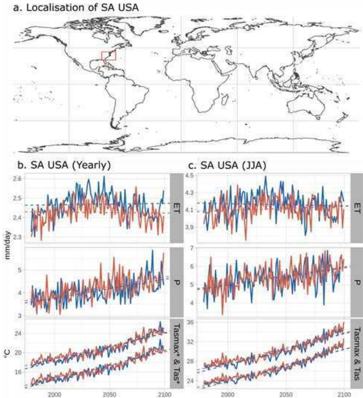
Figure A.7: Localization of USA South Atlantic (SA USA) (a), and regional average values of ET, P, Tas and Tasmax for yearly (b) and JJA means (c) for 1980-2100. Statistical significance of the modulation was tested with a Mann-Kendall test ( p = 0.05 ), and significant trends are shown by a * in the vertical titles. In the Tasmax & Tas panel, the top blue and red lines correspond to Tasmax.
