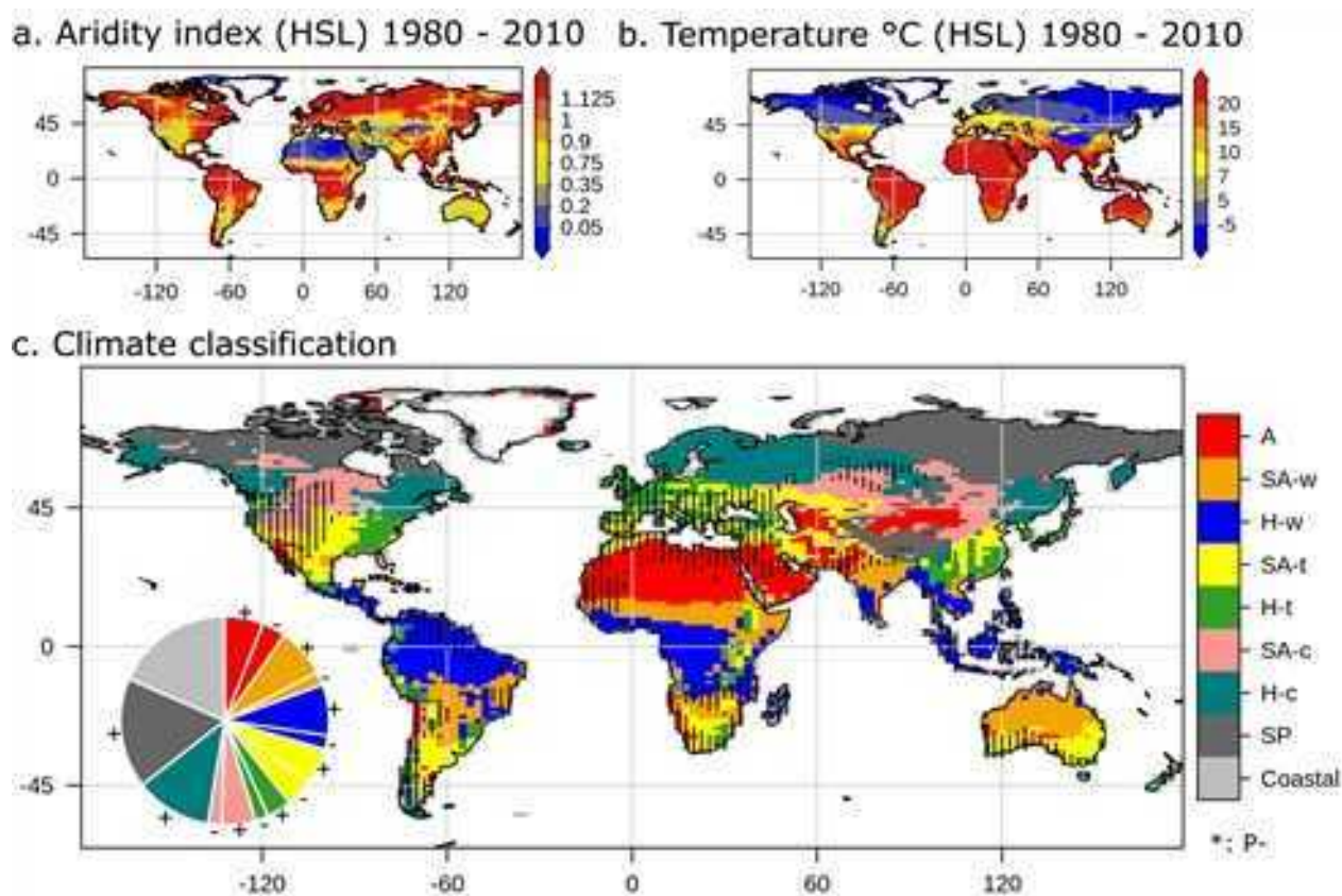
Figure A.8: Aridity index (a), and mean temperature (b) from HSL simulation for period 1980 – 2010. Simple climatic classification from both variables (c). Areas with negative P trends (P-) for the period 1980-2100 are stippled. The piechart shows the distribution of climate classes, separated among positive and negative P trends under climate change (identified by + and -). Climate classes correspond to arid (A), semiarid and warm (SA-w), humid and warm (H-w), semiarid and temperate (SA-t), humid and temperate (H-t), semiarid and cold (SA-c), humid and cold (H-c), and subpolar (SP). Refer to the text in the paper for definition of each class.
