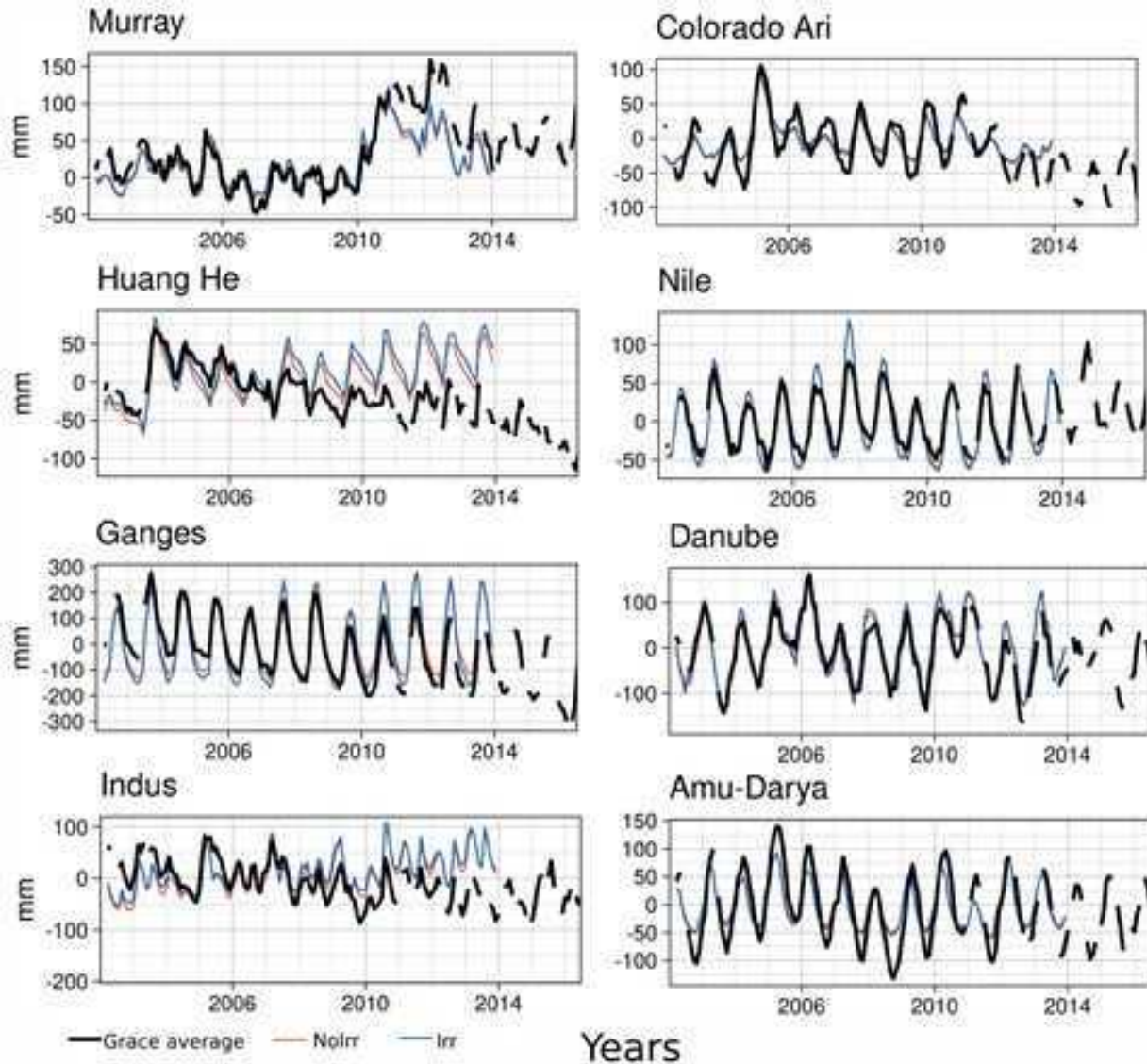
Figure 4.12: Comparison of TWSA between ORCHIDEE simulations and GRACE datasets in large basins with strong irrigation activities.
