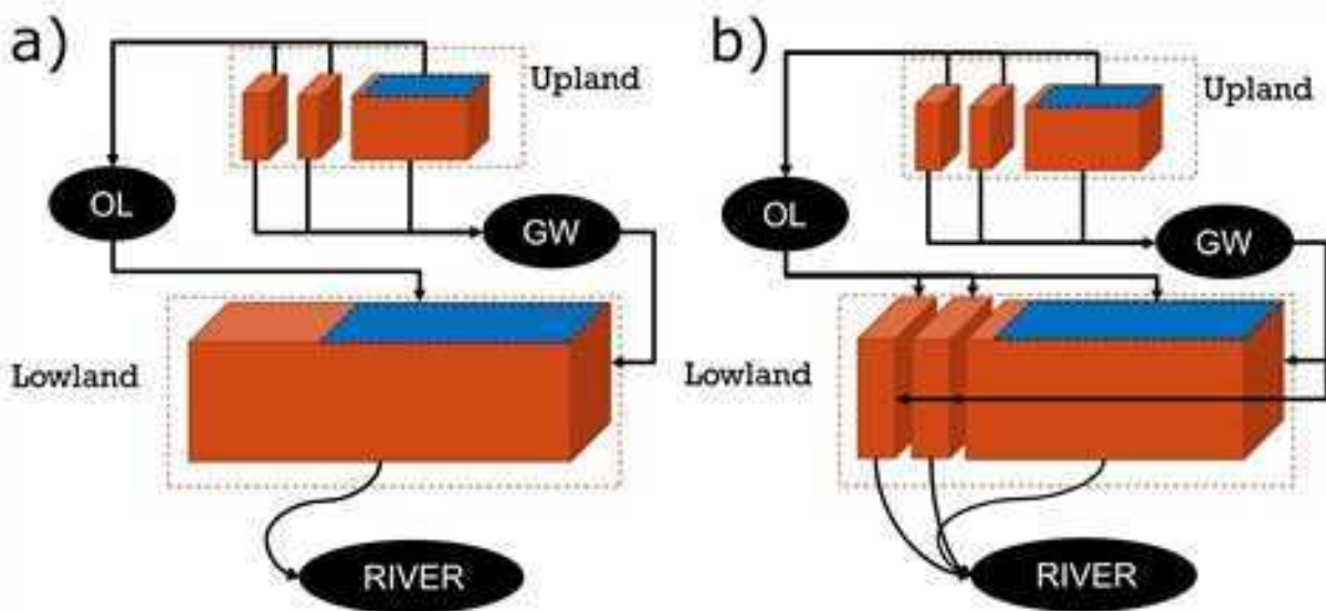
Figure 5.1: Schematic for an ORCHIDEE version with hillslope flow and irrigation. Current hillslope flow representation (a) and new hillslope flow representation (b). The surfaces in blue correspond to the irrigated area, while OL means overland and GW means groundwater reservoirs. Note that for a) there are just 15 PFTs, while for b) there are 30 PFTs.
