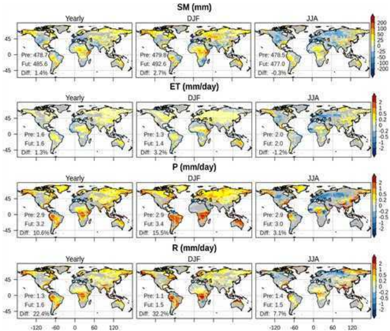
Figure A.3: Change on mean yearly, boreal winter and boreal summer values between periods 2070-2100 and 1980-2100 using REF simulation data, for SM, ET, P and R. Statistical significance of the mean differences is tested at each point with a Student test ( p = 0.05 ). The areas with insignificant changes are left gray
