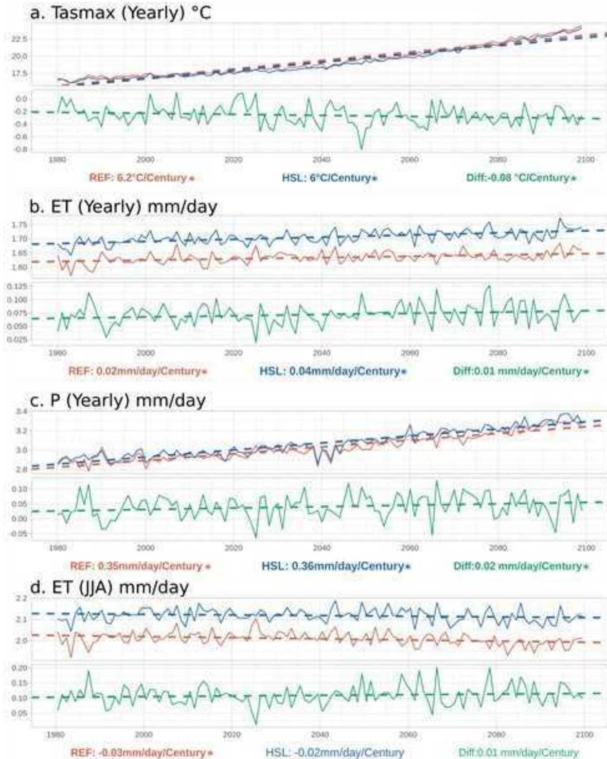
Figure 3.5: Global land average for both simulations, and difference between them, for the period 1980–2100, for daily max. temperature (a), evapotranspiration (b), and precipitation (c), at yearly scale, and evapotranspiration (d) for boreal summer. The statistical significance of the trend was tested with a Mann-Kendall test ( p = 0.05 ). Significant trends are written in bold with an *. Diff. corresponds to the trend of the difference between HSL and REF.
