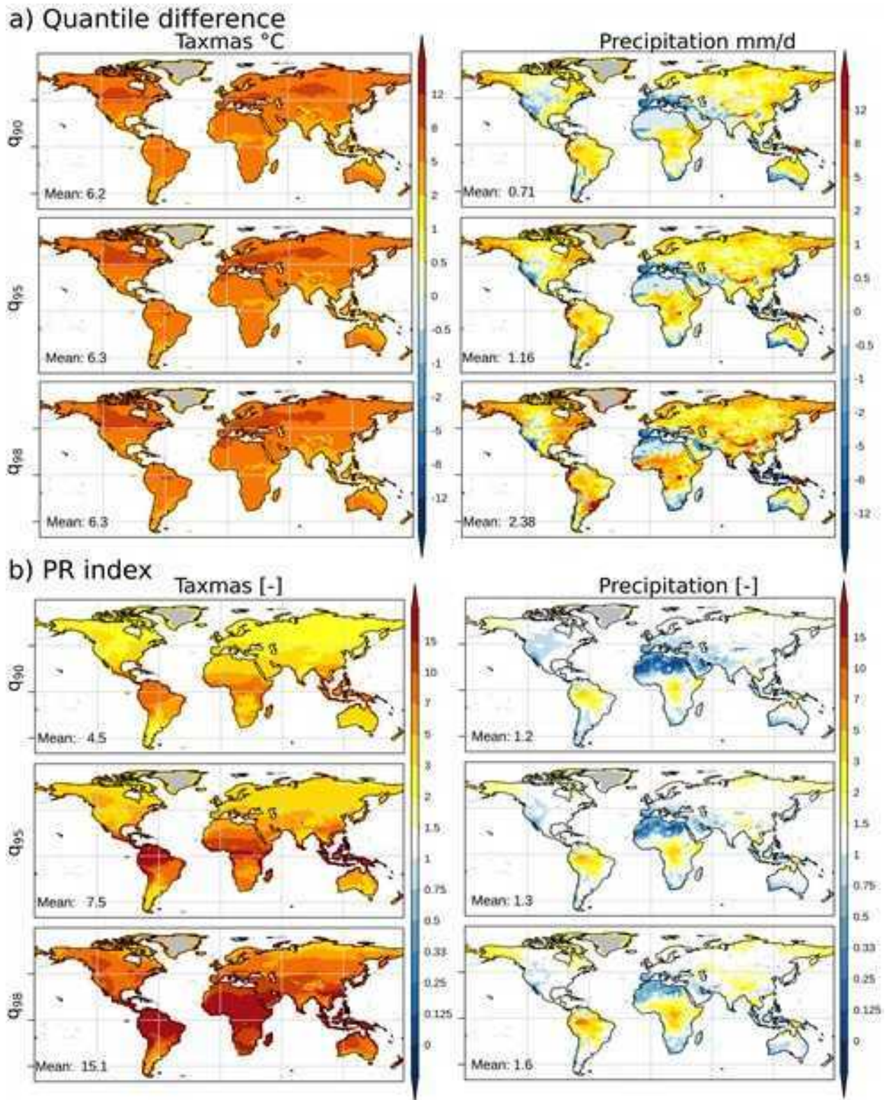
Figure 3.11: Difference of quantiles (a) and PR index (b) between future (2070-2100) and historical (1980-2010), REF simulation, for maximum air temperature Tasmx (first column) and precipitation P (second column).
