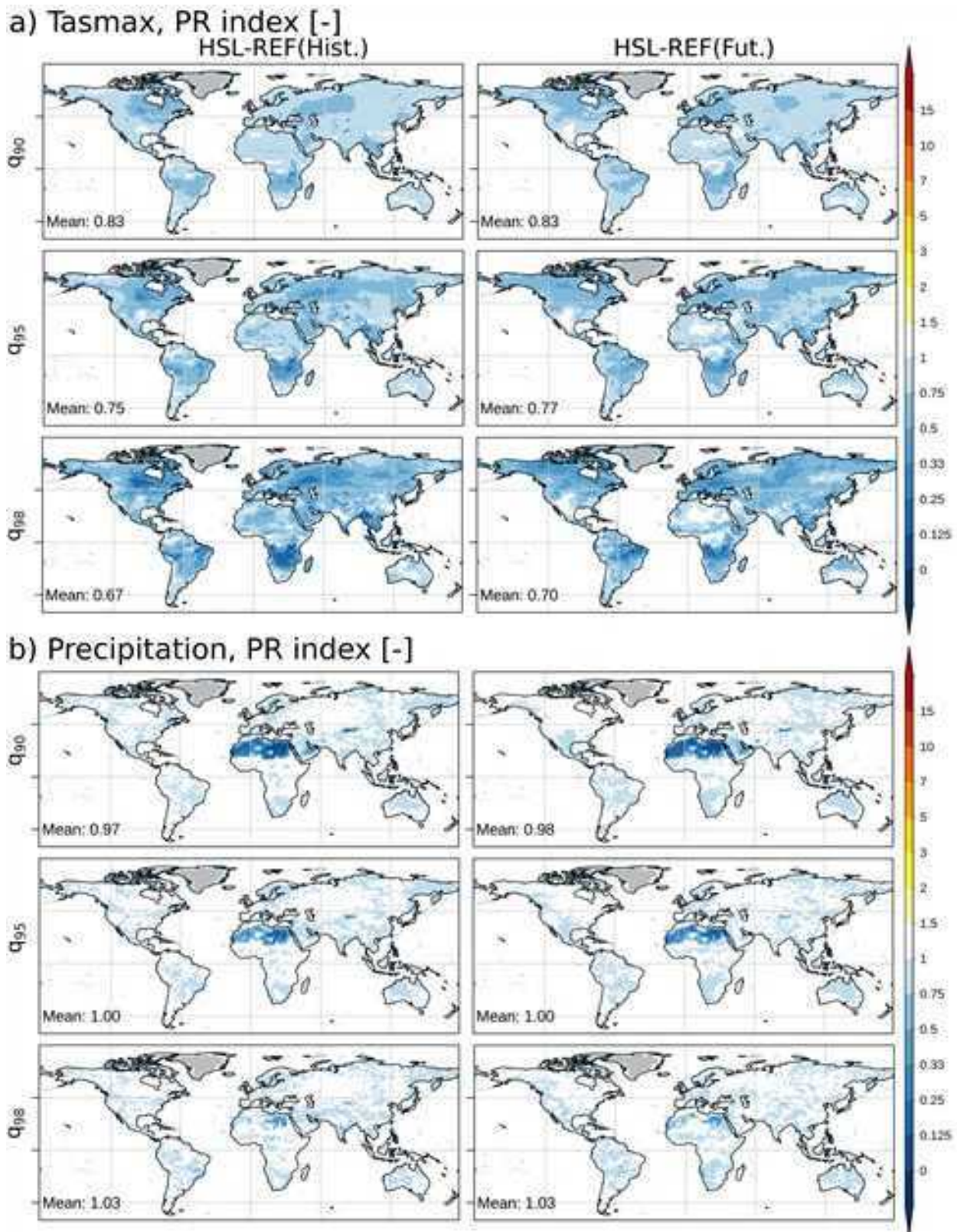
Figure 3.13: PR index for historical (1980-2010, first column) and future (2070-2100, second column) period, between HSL and REF simulations, for maximum air temperature Tasmax (a) and precipitation P (b).
