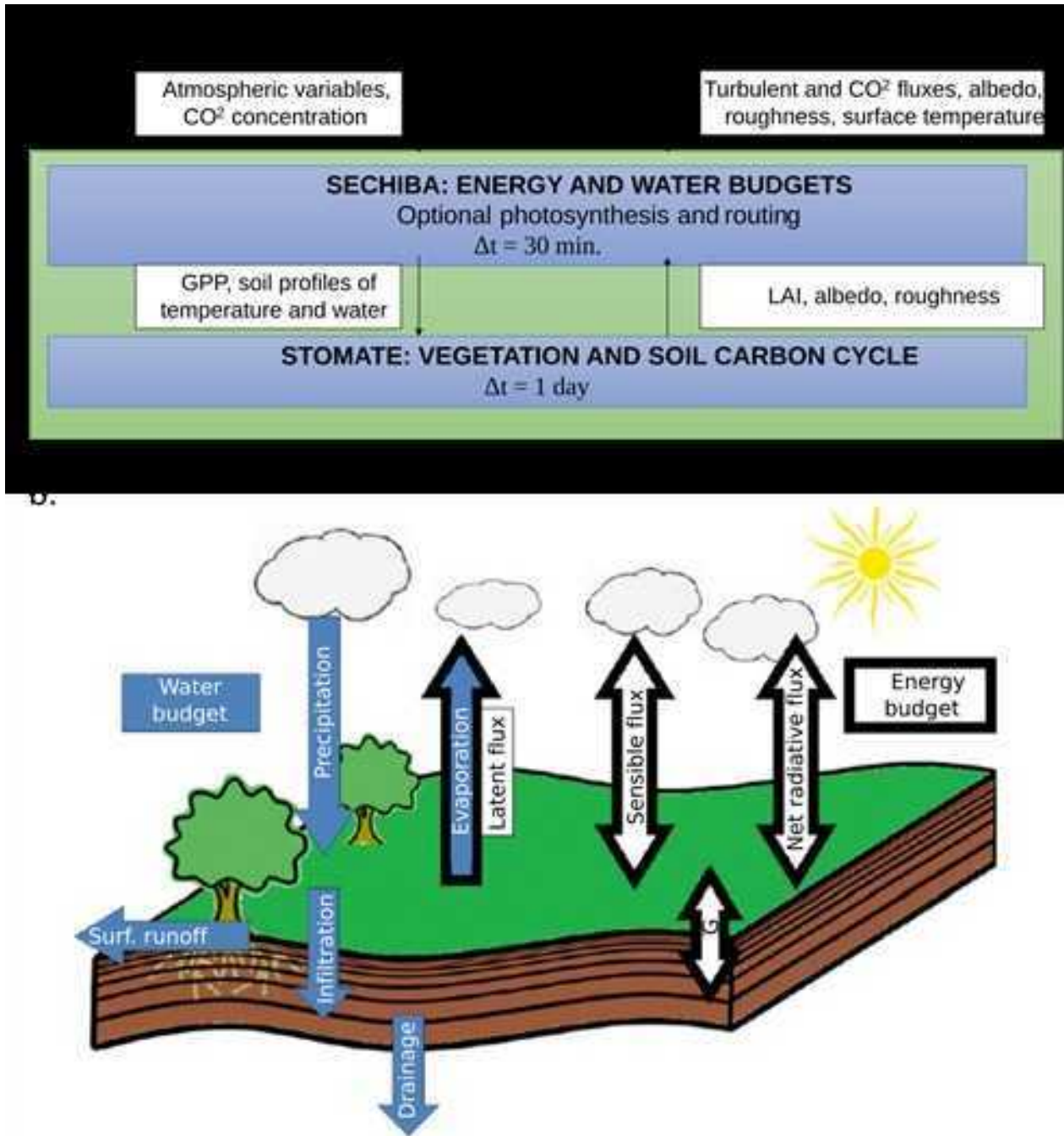
Figure 2.1: Basic structure of ORCHIDEE, depicting SECHIBA and STOMATE coupling. Diagram based on Krinner et al., 2005 and https://orchidee.ipsl.fr/about-orchidee/ with some simplifications (a). GPP mean gross primary production, LAI means leaf area index. Main processes included in ORCHIDEE, water fluxes in blue and energy fluxes in white (b), taken from Campoy et al., 2013. G represents the groundwater flux.
