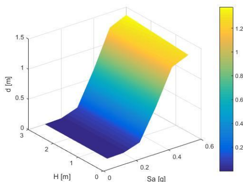
Figure 6. Displacement based on the acceleration and the wave height
