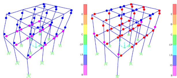
Figure 4. Comparison between support conditions: third degree (a); second degree (b).
