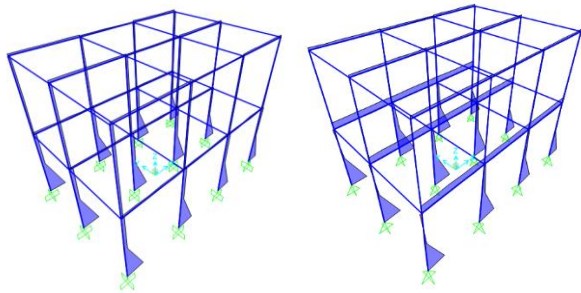
Figure 5. Comparison of shear force with supports of third degree (a) and second degree (b)
