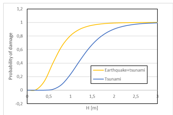
Figure 7. Comparison between fragility curves in collapse damage state Sa=0.5g
