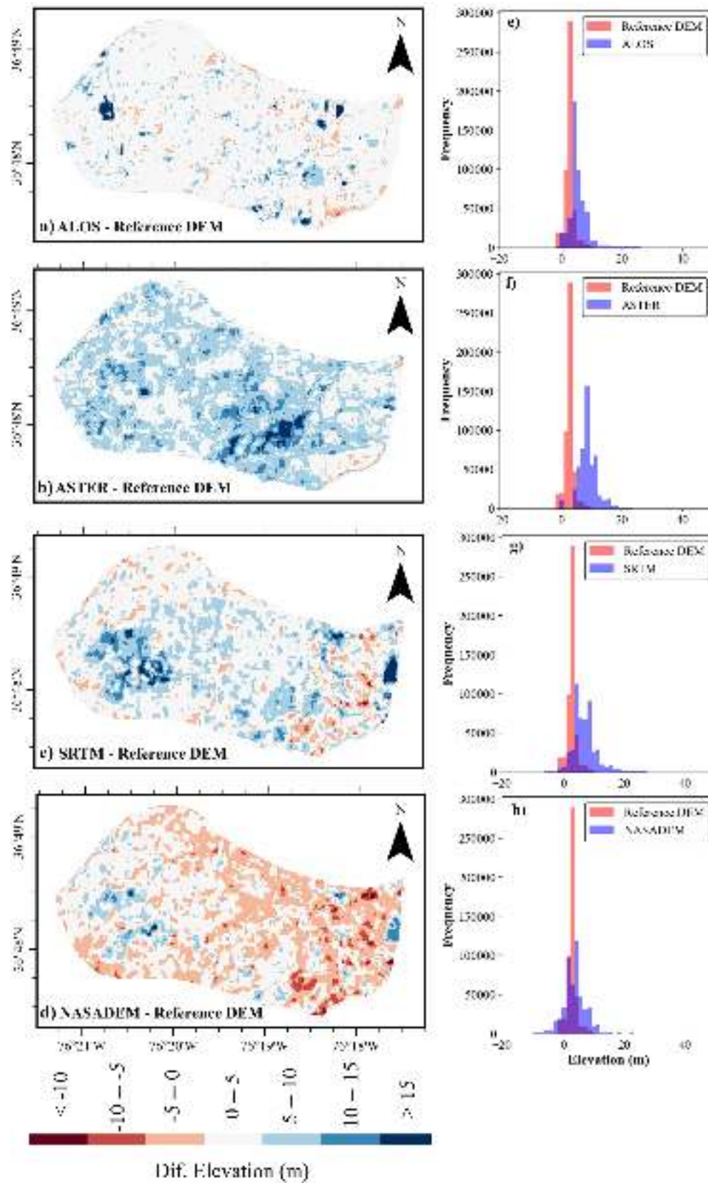
Fig. 4. Comparison between the four GDEMs used in this study (ALOS, ASTER, NASADEM, SRTM) and the reference DEM. (a-d) show the elevation differences between the four GDEMs and the reference DEM. (e-i) compare the frequency distribution of elevation values between the GDEMs and the reference DEM.
