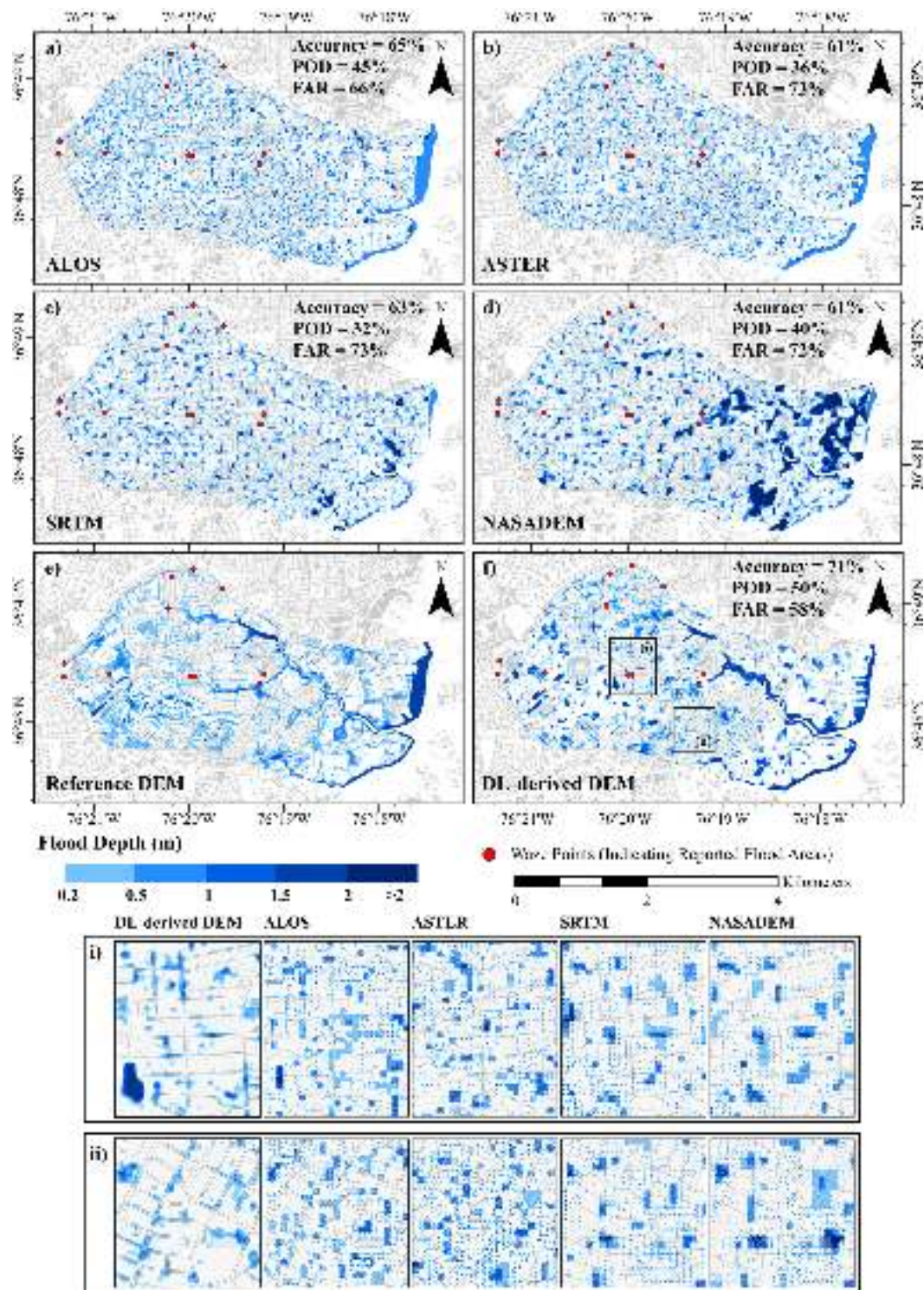
Fig. 7. Comparison of flood inundation extent using different DEMs. (a-d) correspond to ALOS, ASTER, SRTM, and NASADEM, respectively. (e) corresponds to the reference DEM. (f) corresponds to the DL-derived DEM. (i) and (ii) show detailed flood mapping comparisons in road networks in the areas identified in (f).
