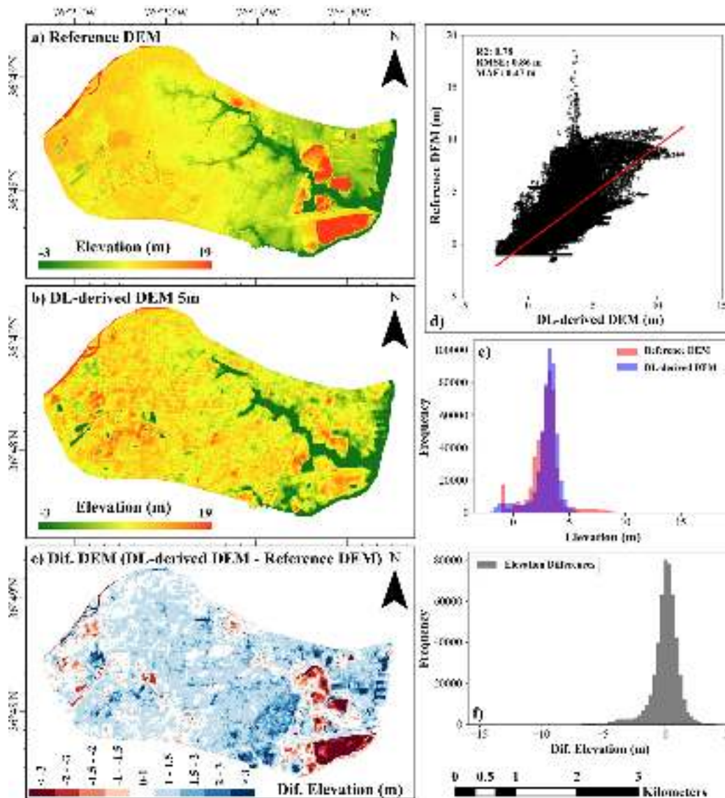
Fig. 5. Comparison between DL-derived DEM and reference DEM. (a) shows the reference DEM over the test area; (b) shows the DL-derived DEM over the test area; (c) shows the elevation difference between the DL-derived and reference DEMs; (d-e) compare the DL-derived DEM with the reference DEM using a scatter plot and a histogram; and (f) shows the histogram of the error (i.e., the difference between DL-derived and reference DEMs).
