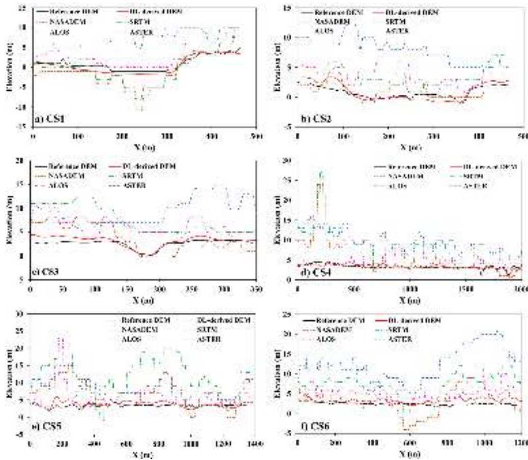
Fig. 6. Elevation profiles in the six cross sections identified in the test watershed based on the four GDEMs, the DL-derived DEM, and the reference DEM.
