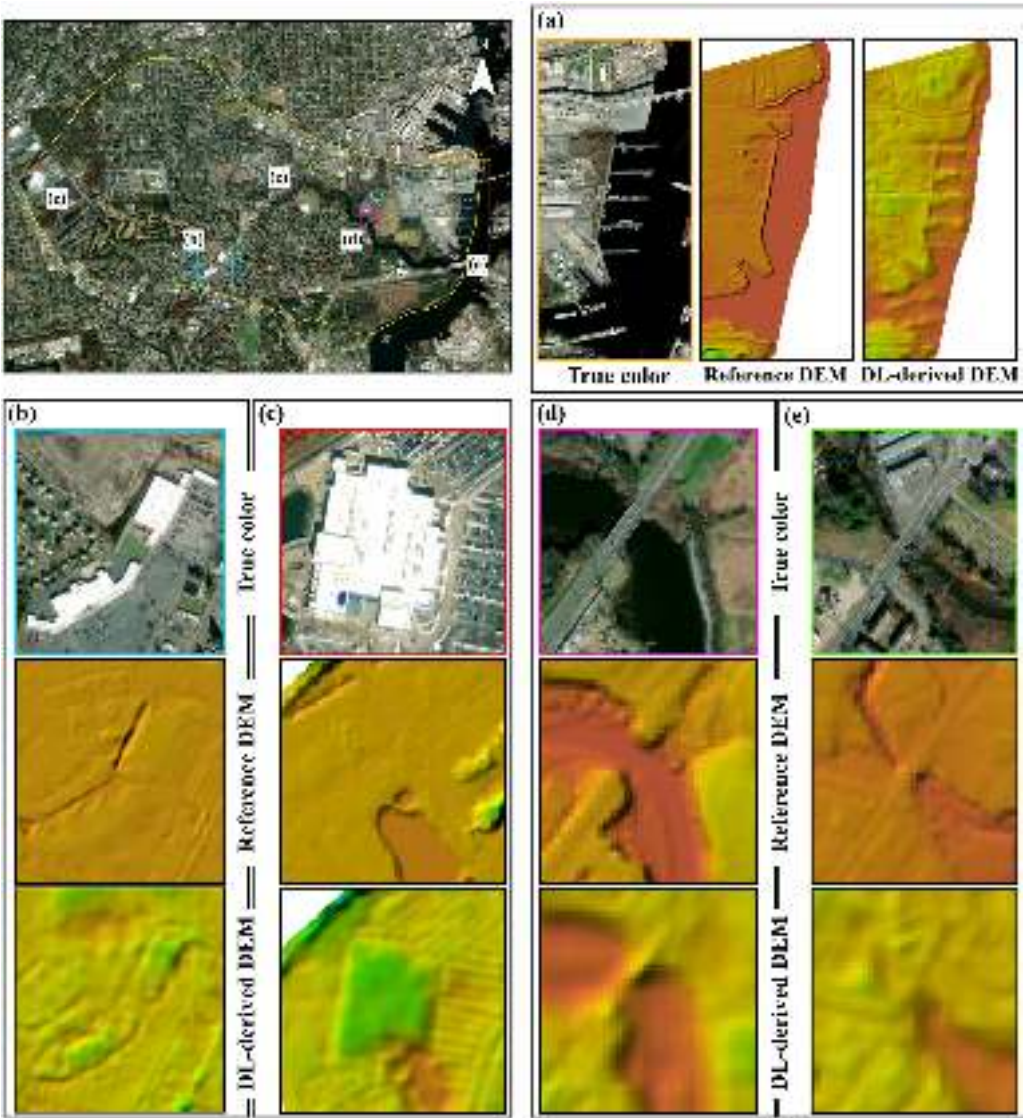
Fig. 8. Visualization of enhanced topographic details using CNN U-Net Model. Each subplot juxtaposes the true-color satellite image with corresponding sections of the reference and DL-derived DEMs, highlighting a terrain feature captured by the DL-derived DEM that is absent in the reference DEM.
