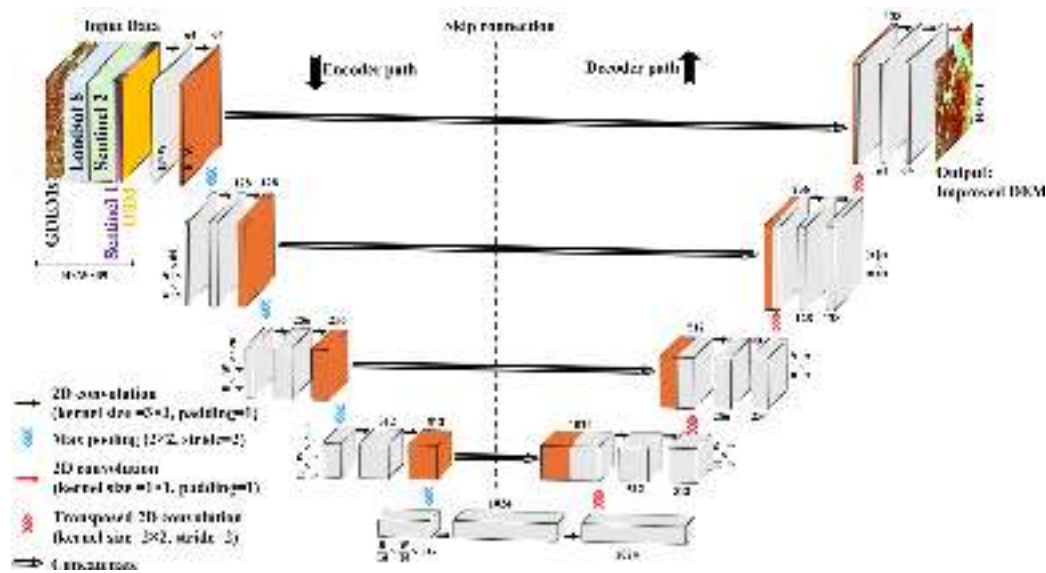
Fig. 2. CNN U-Net architecture for DEM enhancement.
