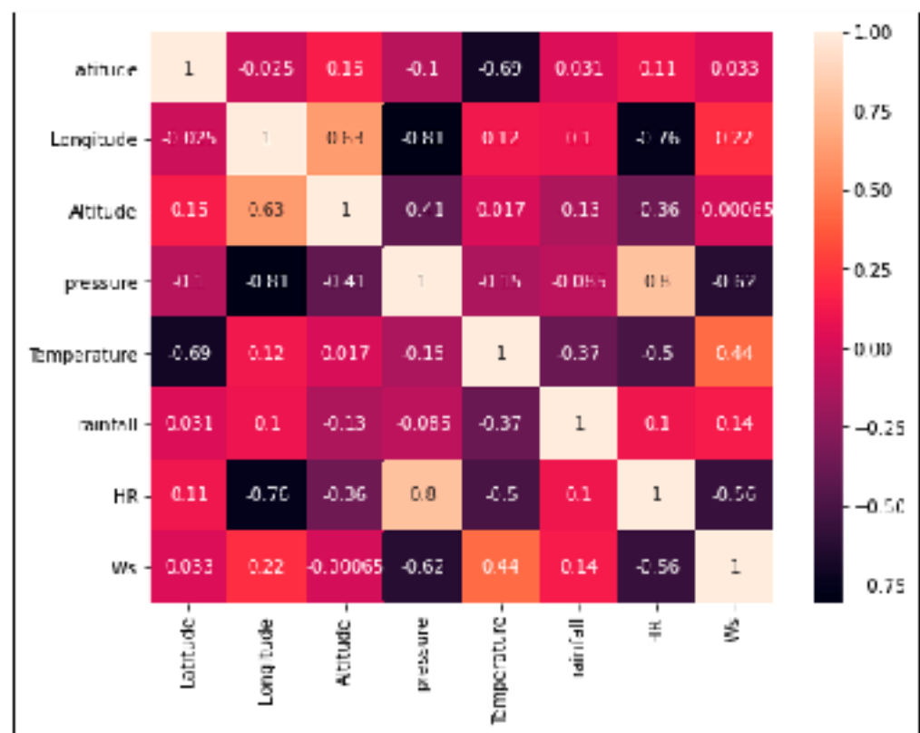
Figure 5. Correlation matrix of Hurst exponents for the time series made up of days with Santa Ana winds.
