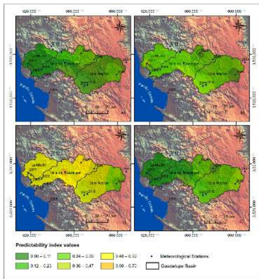
Figure 9. Maps of the predictability index for days with Santa Ana winds for the variables of (a) temperature, (b) pressure, (c) relative humidity, and (d) wind speed.
