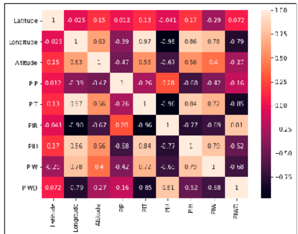
Figure 4. Correlation matrix for predictability indices for the time series made up of days without Santa Ana winds.
