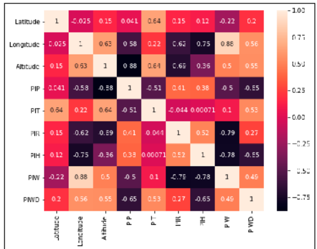
Figure 3. Correlation matrix for predictability indices for the time series made up of days with Santa Ana winds.
